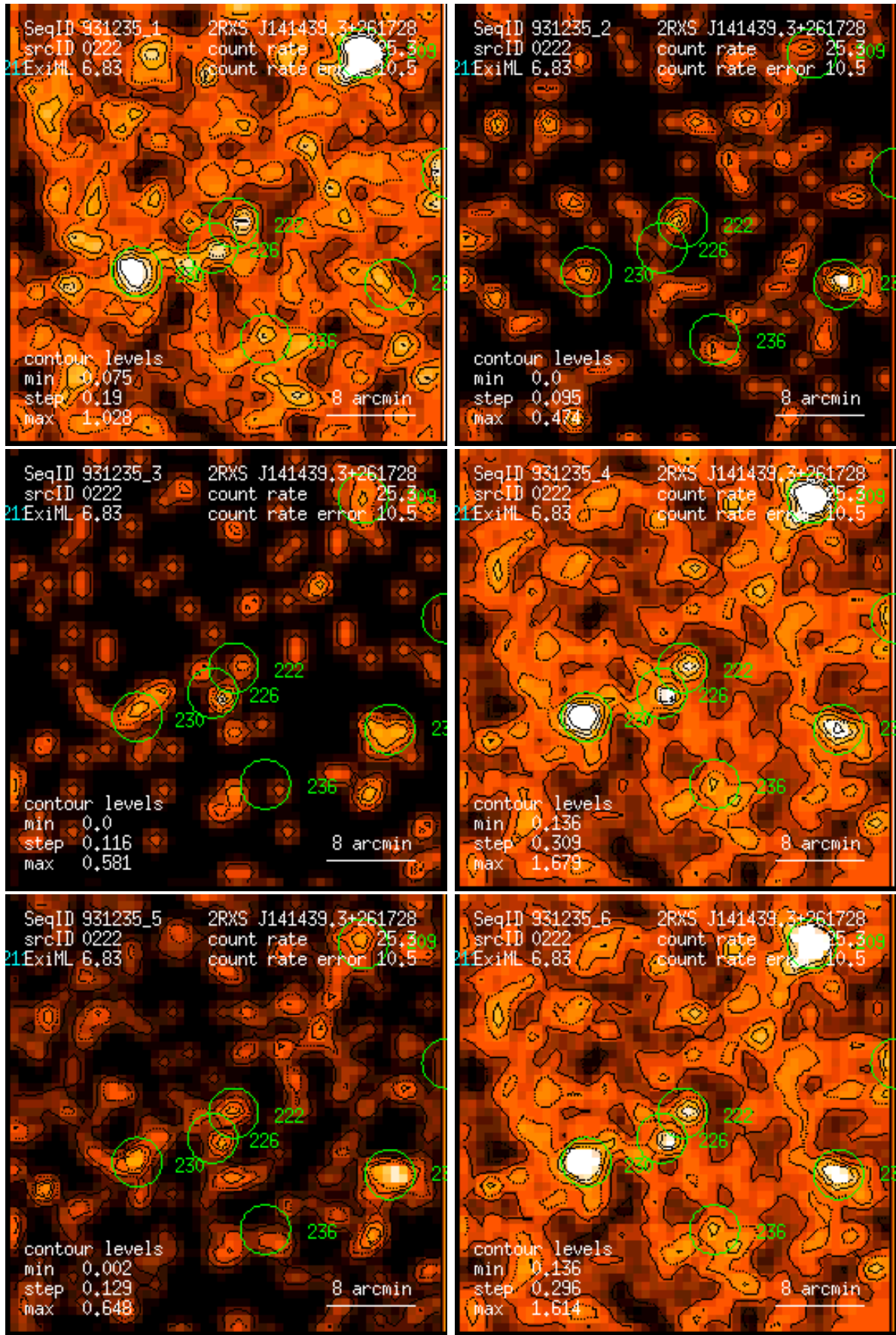
Figure 222: RASS 931235: detection 0222: band rate images, Gaussian filter: (1) PSPC channels 11 – 41, (2) 52 – 90, (3) 91 – 201, (4) 11 – 235, (5) 52 – 201, (6) 11 – 201. Broad band rates in counts/ks. Band rate contour levels in counts/ks/arcmin 2 .
