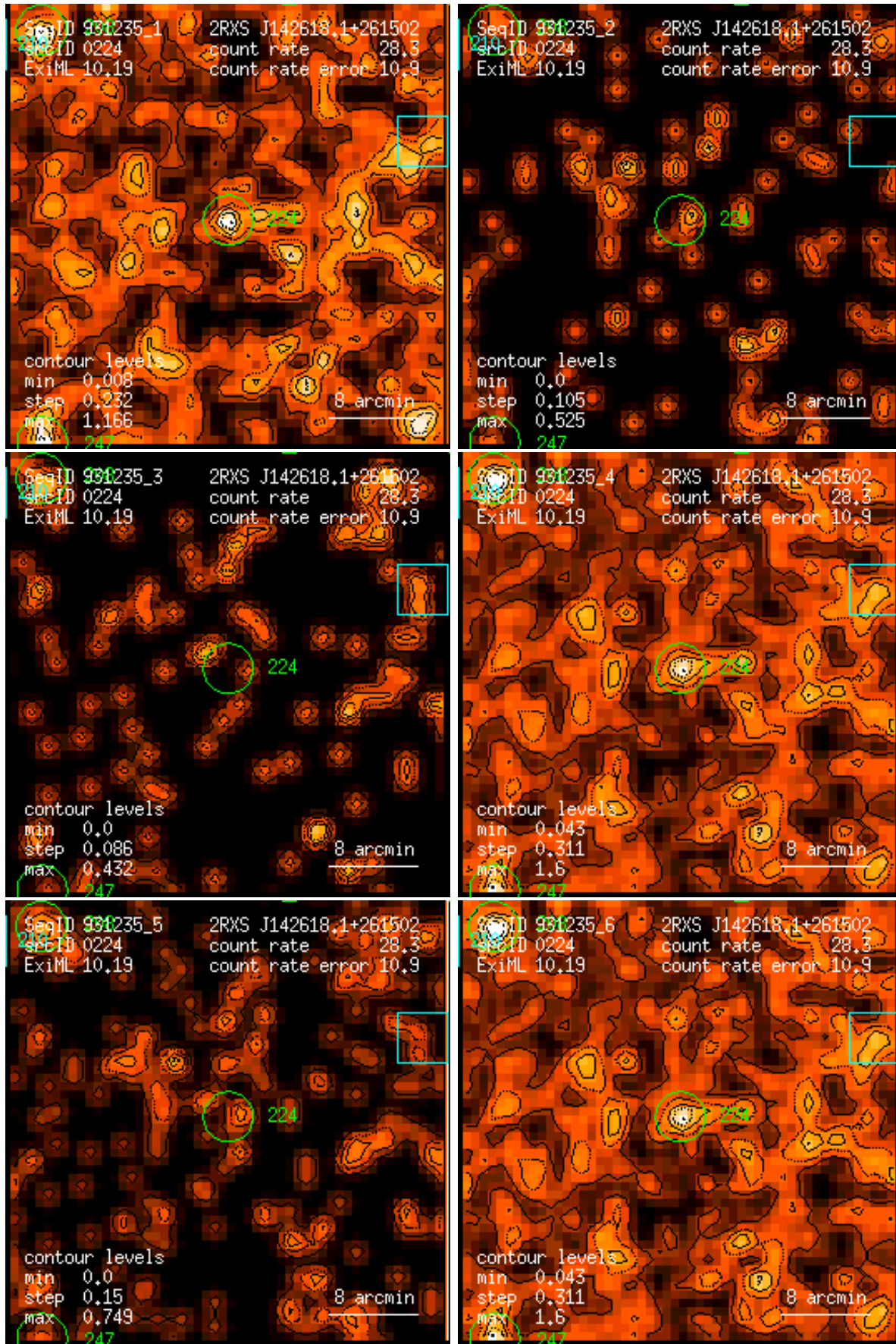
Figure 224: RASS 931235: detection 0224: band rate images, Gaussian filter: (1) PSPC channels 11 – 41, (2) 52 – 90, (3) 91 – 201, (4) 11 – 235, (5) 52 – 201, (6) 11 – 201. Broad band rates in counts/ks. Band rate contour levels in counts/ks/arcmin 2 .
