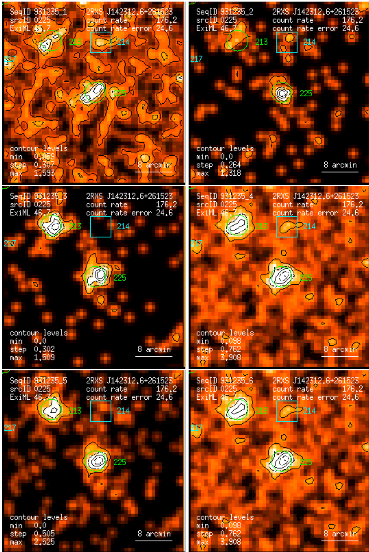
Figure 225: RASS 931235: detection 0225: band rate images, Gaussian filter: (1) PSPC channels 11 – 41, (2) 52 – 90, (3) 91 – 201, (4) 11 – 235, (5) 52 – 201, (6) 11 – 201. Broad band rates in counts/ks. Band rate contour levels in counts/ks/arcmin 2 .
