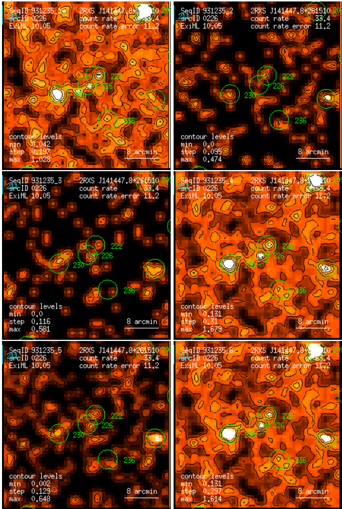
Figure 226: RASS 931235: detection 0226: band rate images, Gaussian filter: (1) PSPC channels 11 – 41, (2) 52 – 90, (3) 91 – 201, (4) 11 – 235, (5) 52 – 201, (6) 11 – 201. Broad band rates in counts/ks. Band rate contour levels in counts/ks/arcmin 2 .
