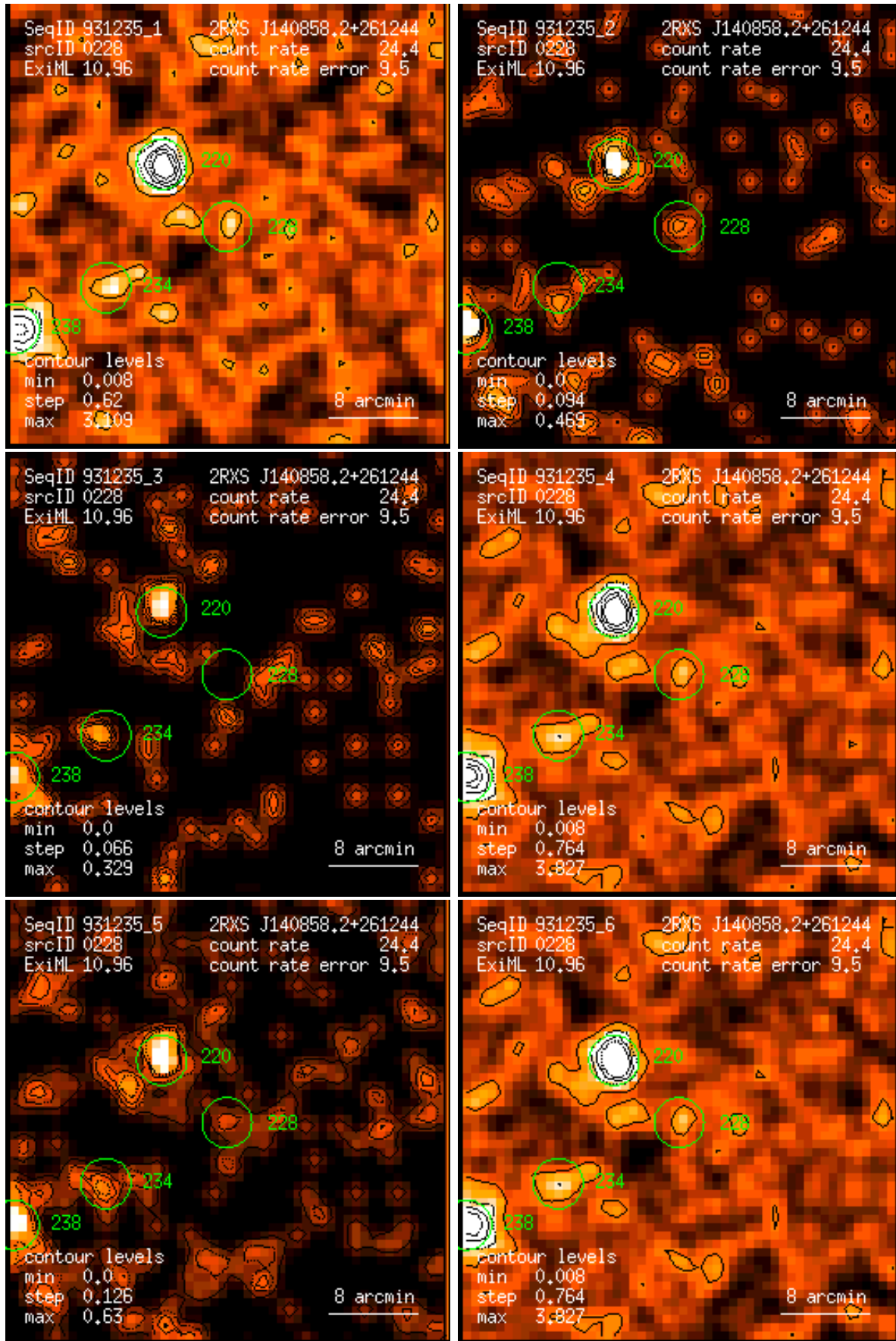
Figure 228: RASS 931235: detection 0228: band rate images, Gaussian filter: (1) PSPC channels 11 – 41, (2) 52 – 90, (3) 91 – 201, (4) 11 – 235, (5) 52 – 201, (6) 11 – 201. Broad band rates in counts/ks. Band rate contour levels in counts/ks/arcmin 2 .
