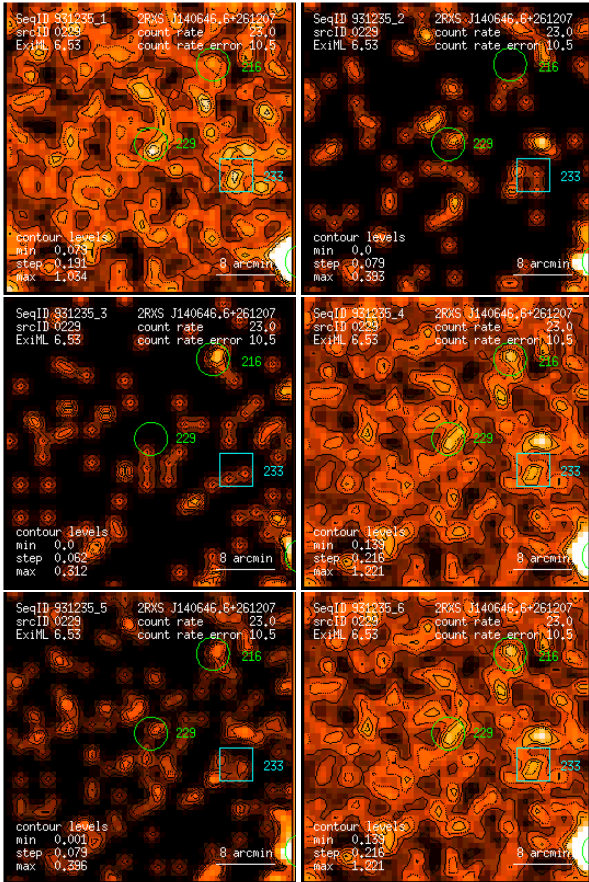
Figure 229: RASS 931235: detection 0229: band rate images, Gaussian filter: (1) PSPC channels 11 – 41, (2) 52 – 90, (3) 91 – 201, (4) 11 – 235, (5) 52 – 201, (6) 11 – 201. Broad band rates in counts/ks. Band rate contour levels in counts/ks/arcmin 2 .
