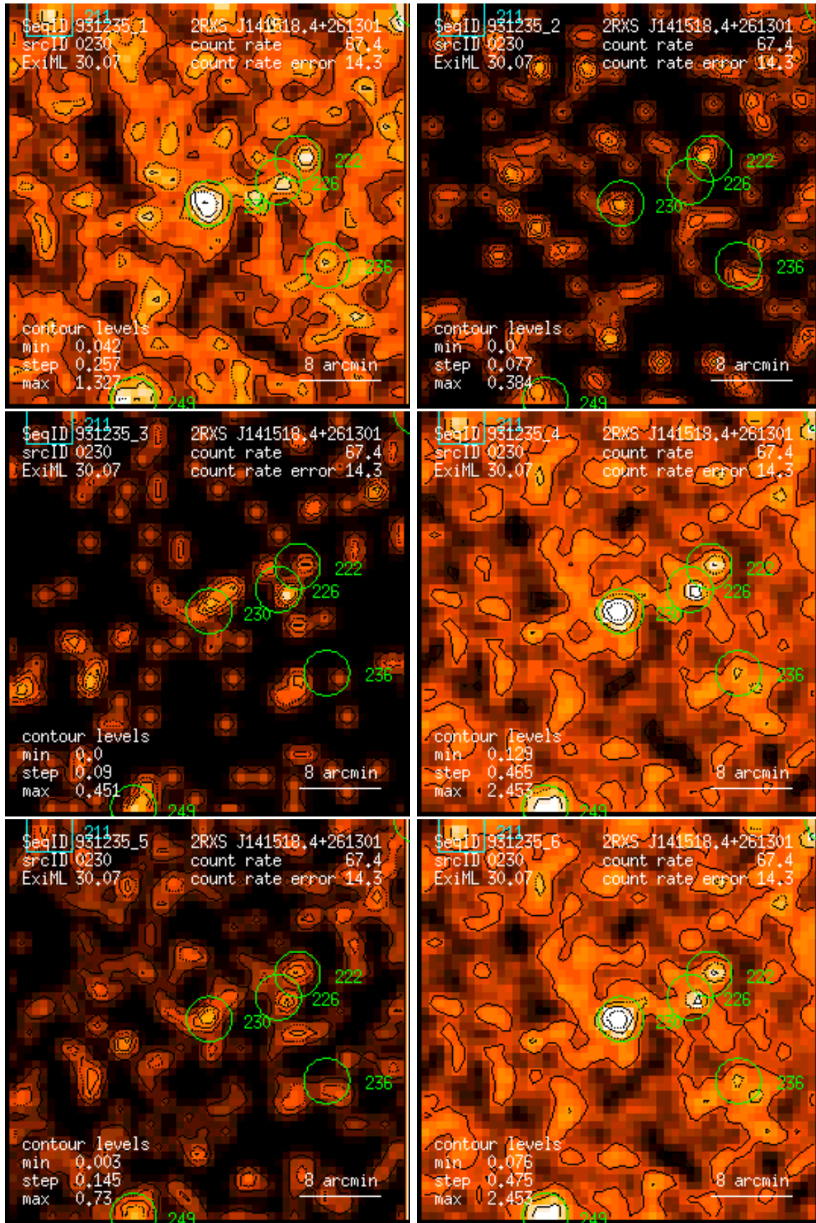
Figure 230: RASS 931235: detection 0230: band rate images, Gaussian filter: (1) PSPC channels 11 – 41, (2) 52 – 90, (3) 91 – 201, (4) 11 – 235, (5) 52 – 201, (6) 11 – 201. Broad band rates in counts/ks. Band rate contour levels in counts/ks/arcmin 2 .
