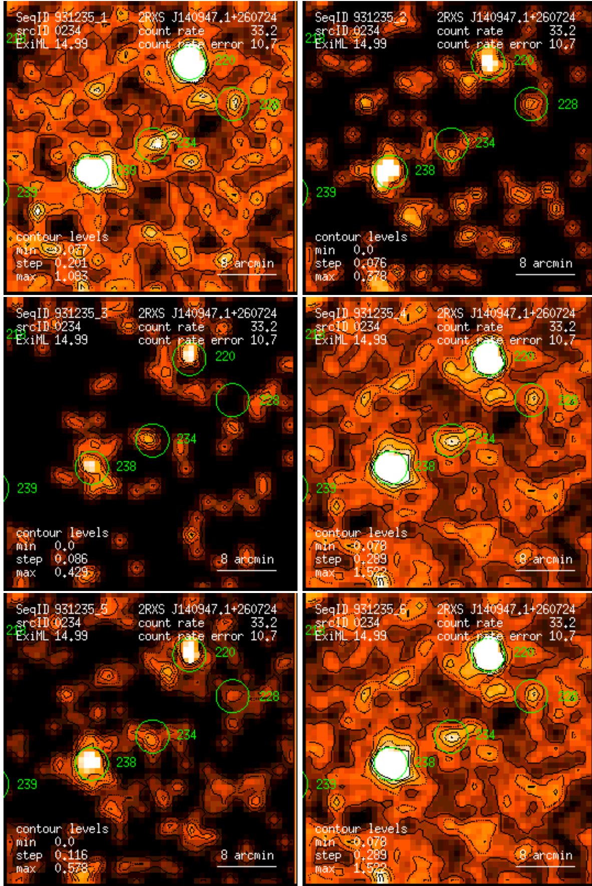
Figure 234: RASS 931235: detection 0234: band rate images, Gaussian filter: (1) PSPC channels 11 – 41, (2) 52 – 90, (3) 91 – 201, (4) 11 – 235, (5) 52 – 201, (6) 11 – 201. Broad band rates in counts/ks. Band rate contour levels in counts/ks/arcmin 2 .
