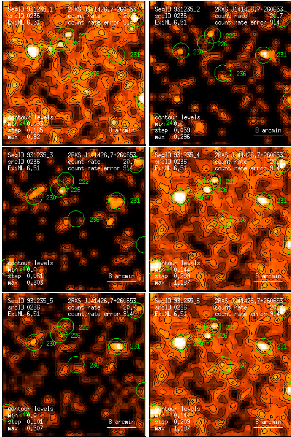
Figure 236: RASS 931235: detection 0236: band rate images, Gaussian filter: (1) PSPC channels 11 – 41, (2) 52 – 90, (3) 91 – 201, (4) 11 – 235, (5) 52 – 201, (6) 11 – 201. Broad band rates in counts/ks. Band rate contour levels in counts/ks/arcmin 2 .
