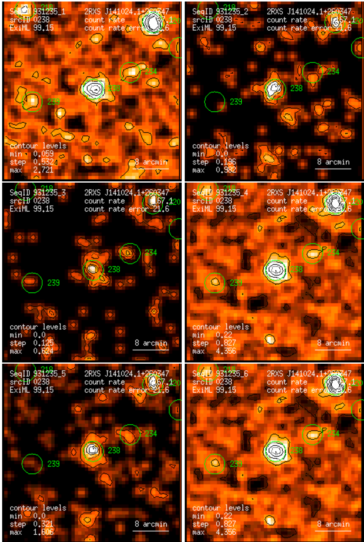
Figure 238: RASS 931235: detection 0238: band rate images, Gaussian filter: (1) PSPC channels 11 – 41, (2) 52 – 90, (3) 91 – 201, (4) 11 – 235, (5) 52 – 201, (6) 11 – 201. Broad band rates in counts/ks. Band rate contour levels in counts/ks/arcmin 2 .
