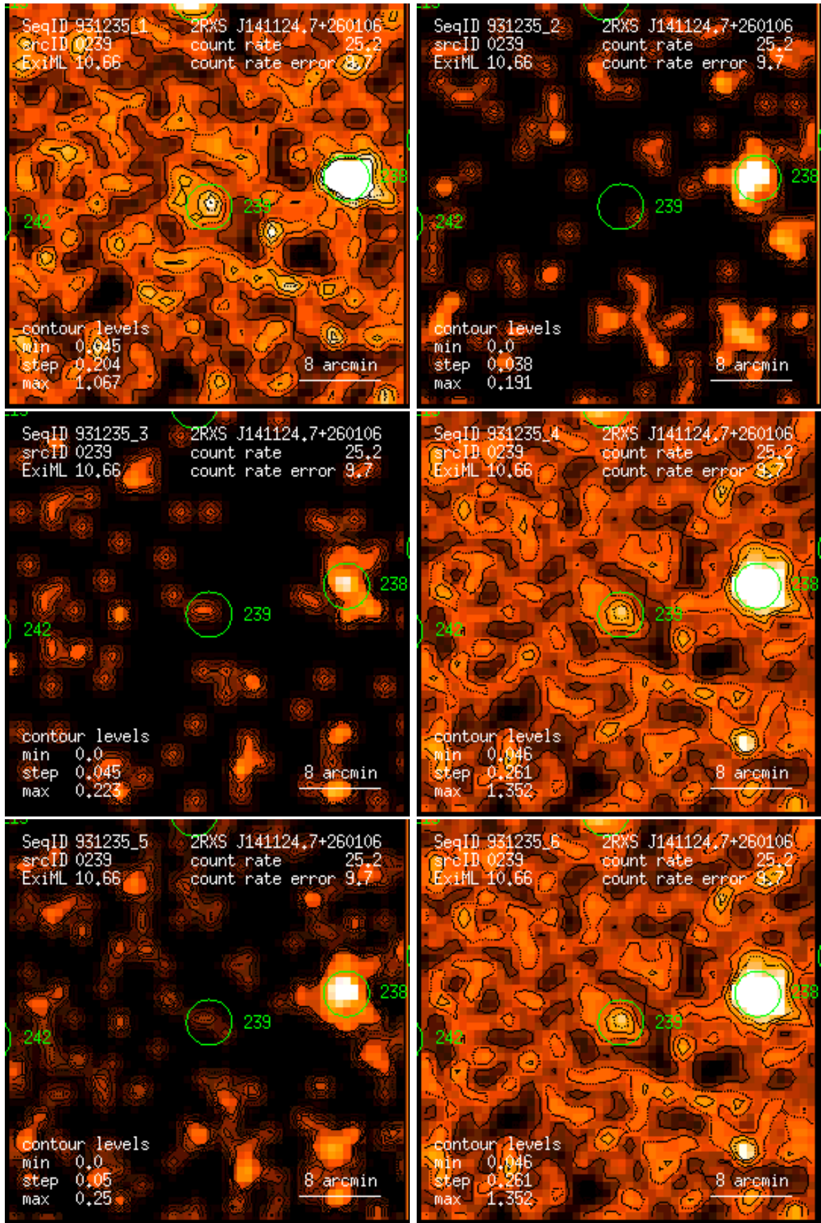
Figure 239: RASS 931235: detection 0239: band rate images, Gaussian filter: (1) PSPC channels 11 – 41, (2) 52 – 90, (3) 91 – 201, (4) 11 – 235, (5) 52 – 201, (6) 11 – 201. Broad band rates in counts/ks. Band rate contour levels in counts/ks/arcmin 2 .
