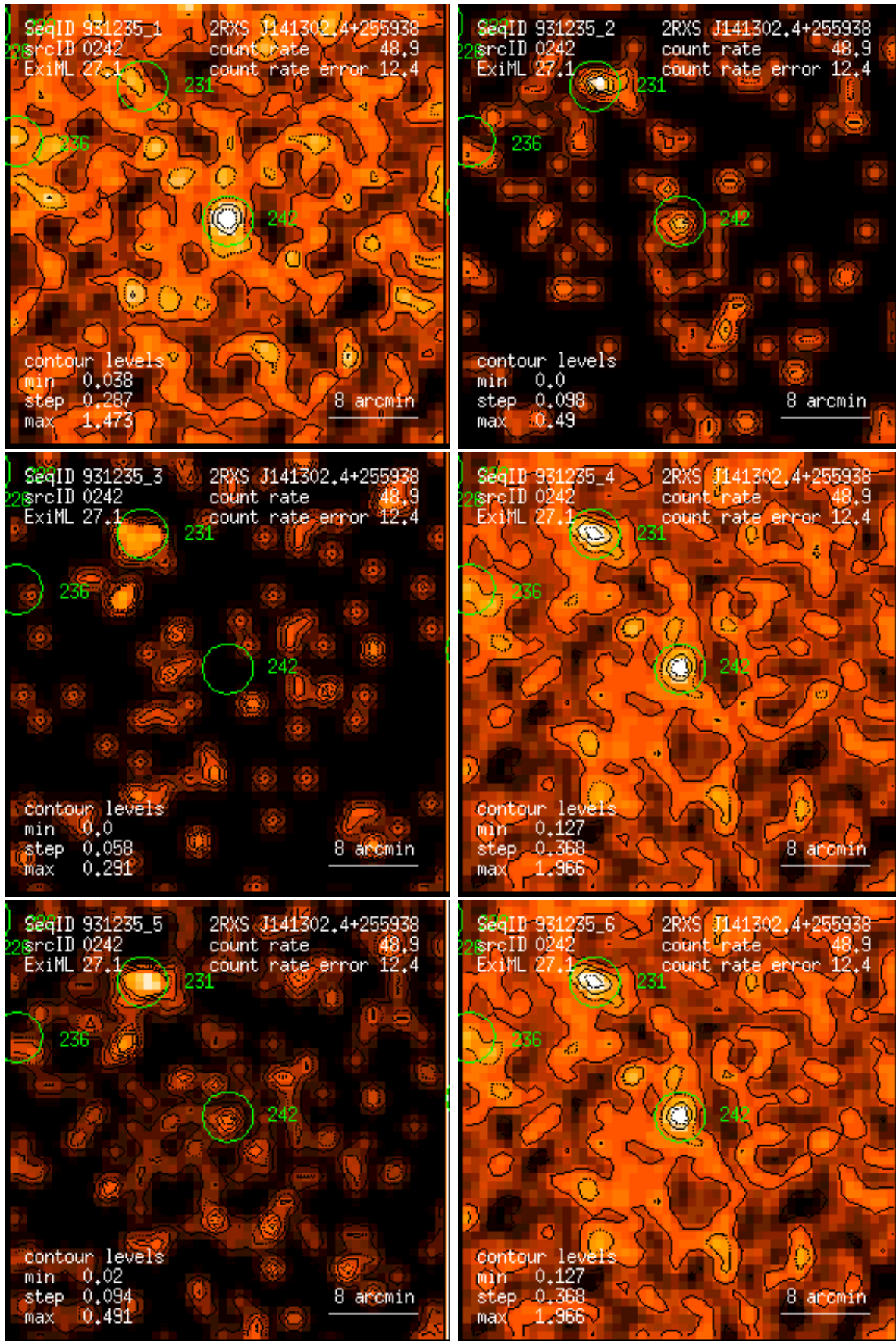
Figure 242: RASS 931235: detection 0242: band rate images, Gaussian filter: (1) PSPC channels 11 – 41, (2) 52 – 90, (3) 91 – 201, (4) 11 – 235, (5) 52 – 201, (6) 11 – 201. Broad band rates in counts/ks. Band rate contour levels in counts/ks/arcmin 2 .
