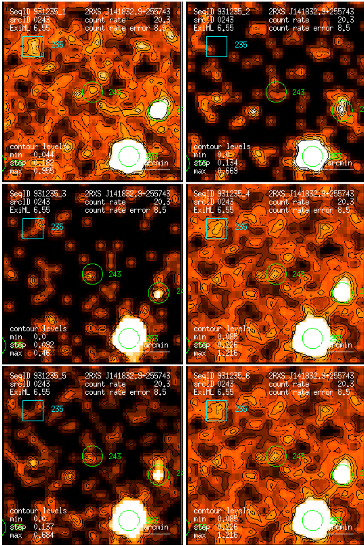
Figure 243: RASS 931235: detection 0243: band rate images, Gaussian filter: (1) PSPC channels 11 – 41, (2) 52 – 90, (3) 91 – 201, (4) 11 – 235, (5) 52 – 201, (6) 11 – 201. Broad band rates in counts/ks. Band rate contour levels in counts/ks/arcmin 2 .
