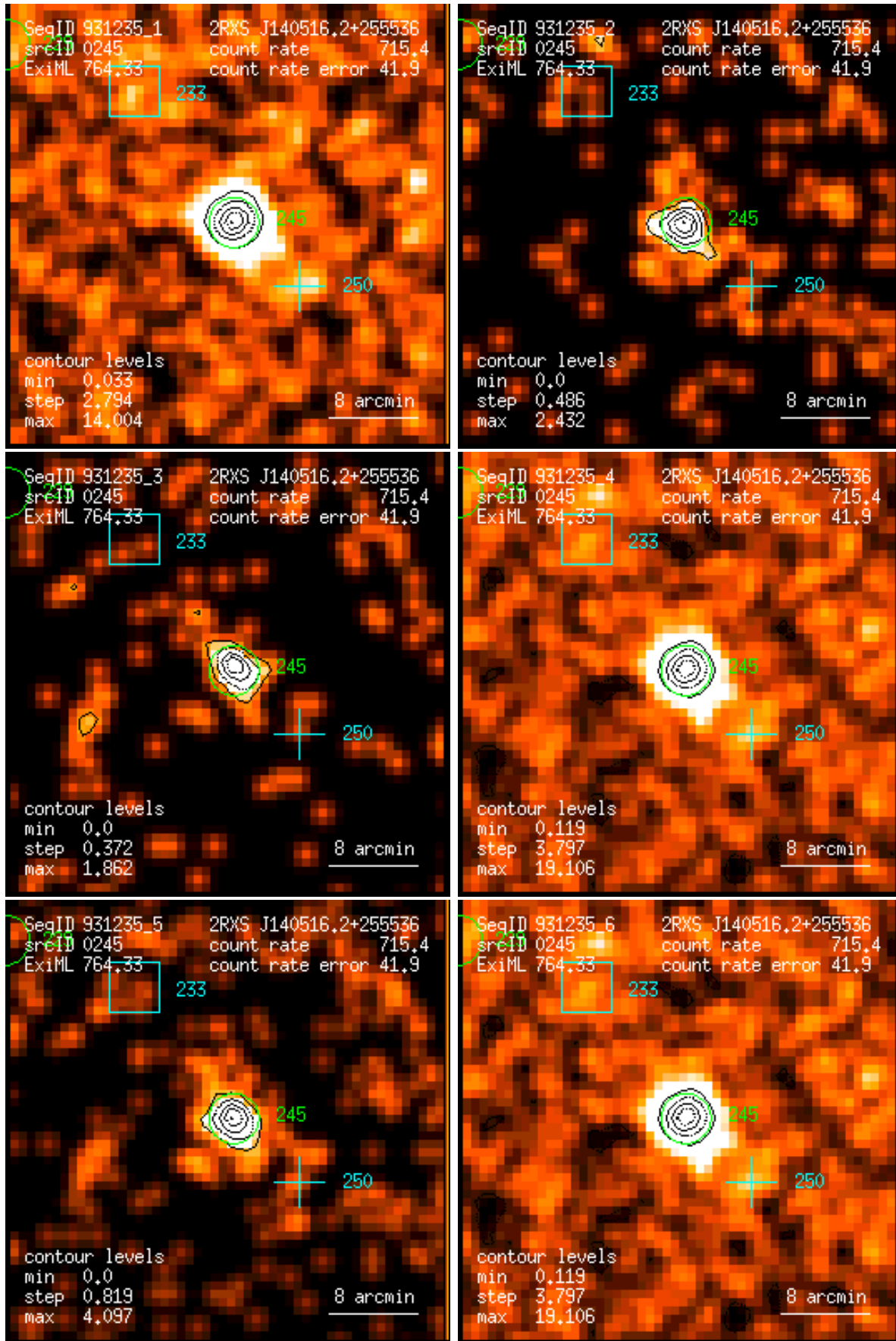
Figure 245: RASS 931235: detection 0245: band rate images, Gaussian filter: (1) PSPC channels 11 – 41, (2) 52 – 90, (3) 91 – 201, (4) 11 – 235, (5) 52 – 201, (6) 11 – 201. Broad band rates in counts/ks. Band rate contour levels in counts/ks/arcmin 2 .
