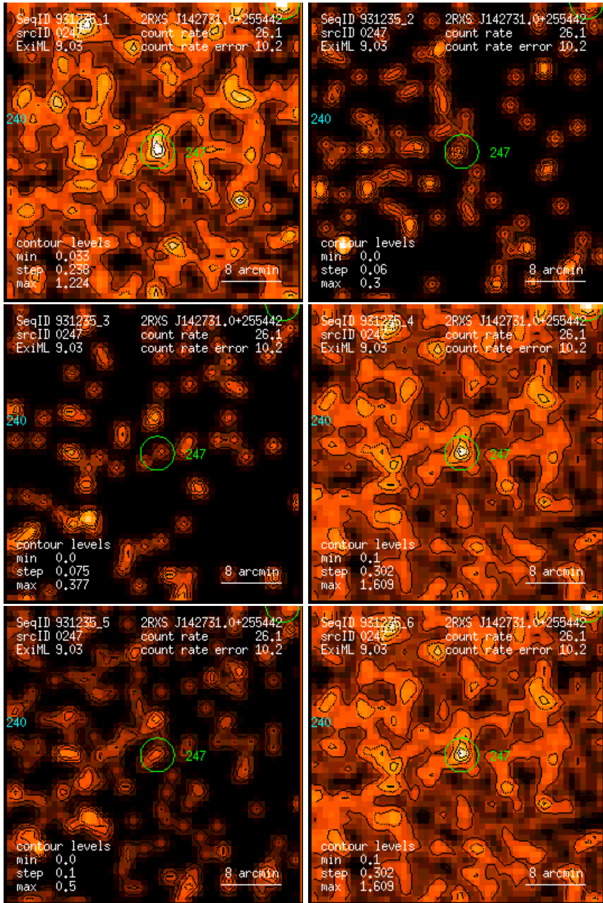
Figure 247: RASS 931235: detection 0247: band rate images, Gaussian filter: (1) PSPC channels 11 – 41, (2) 52 – 90, (3) 91 – 201, (4) 11 – 235, (5) 52 – 201, (6) 11 – 201. Broad band rates in counts/ks. Band rate contour levels in counts/ks/arcmin 2 .
