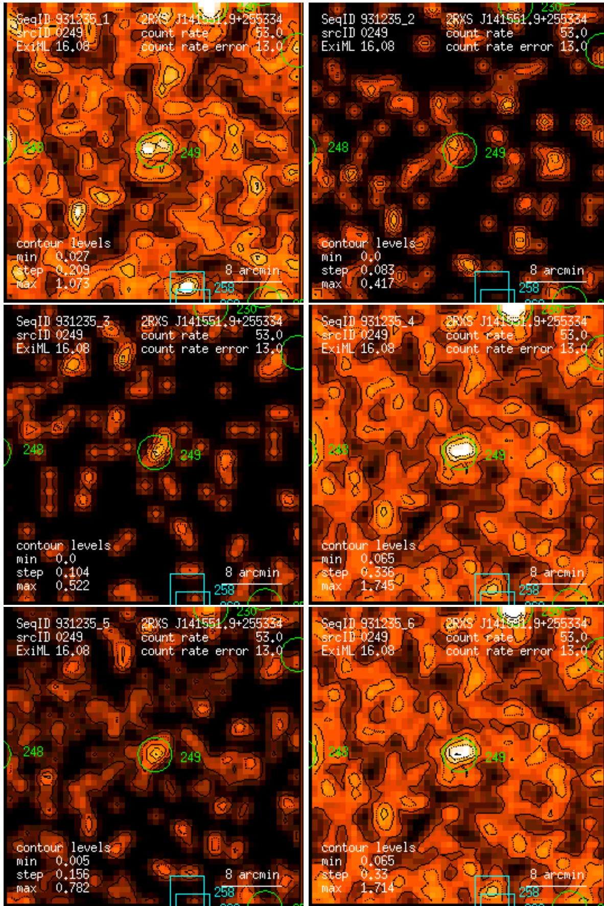
Figure 249: RASS 931235: detection 0249: band rate images, Gaussian filter: (1) PSPC channels 11 – 41, (2) 52 – 90, (3) 91 – 201, (4) 11 – 235, (5) 52 – 201, (6) 11 – 201. Broad band rates in counts/ks. Band rate contour levels in counts/ks/arcmin 2 .
