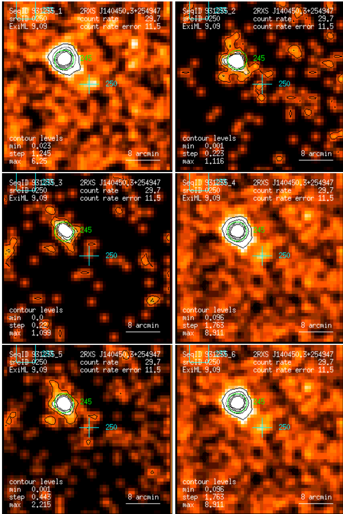
Figure 250: RASS 931235: detection 0250: band rate images, Gaussian filter: (1) PSPC channels 11 – 41, (2) 52 – 90, (3) 91 – 201, (4) 11 – 235, (5) 52 – 201, (6) 11 – 201. Broad band rates in counts/ks. Band rate contour levels in counts/ks/arcmin 2 .
