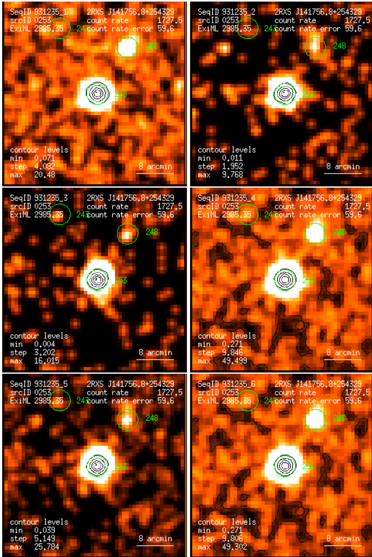
Figure 253: RASS 931235: detection 0253: band rate images, Gaussian filter: (1) PSPC channels 11 – 41, (2) 52 – 90, (3) 91 – 201, (4) 11 – 235, (5) 52 – 201, (6) 11 – 201. Broad band rates in counts/ks. Band rate contour levels in counts/ks/arcmin 2 .
