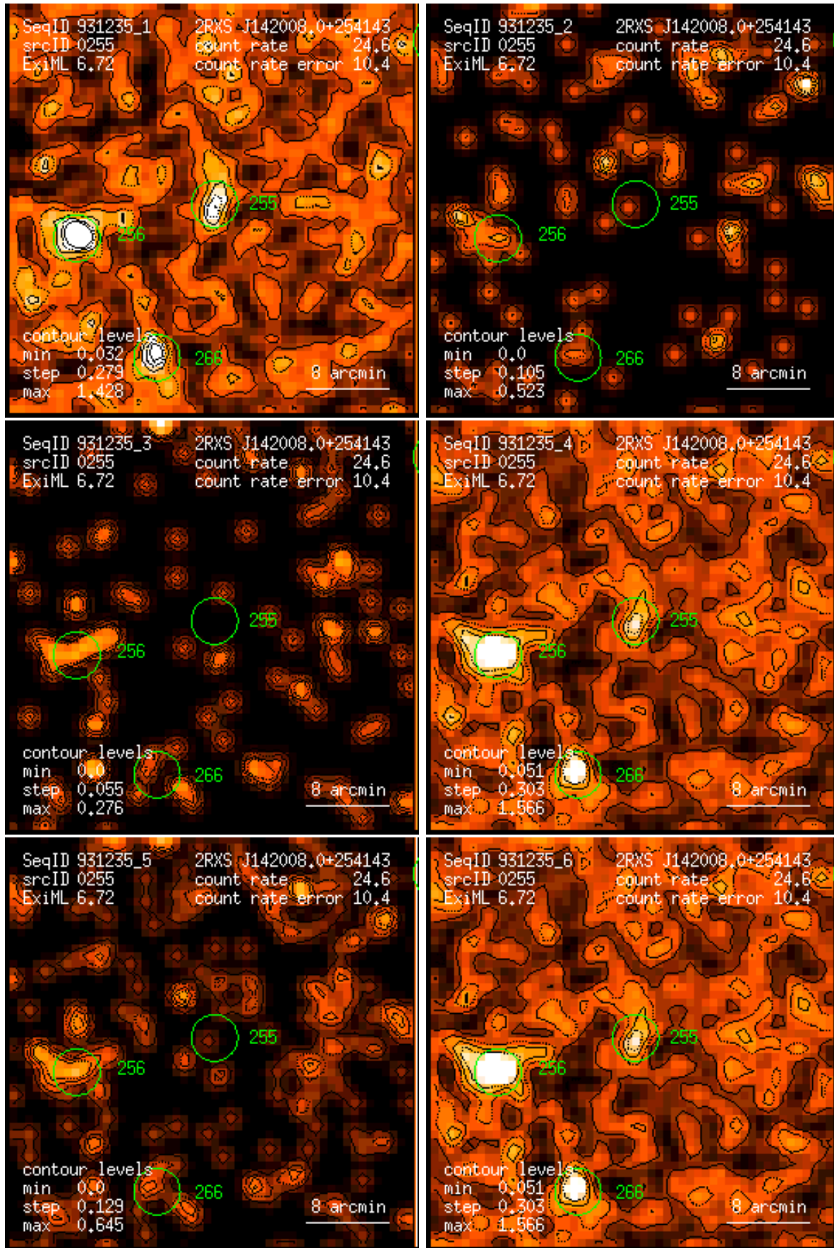
Figure 255: RASS 931235: detection 0255: band rate images, Gaussian filter: (1) PSPC channels 11 – 41, (2) 52 – 90, (3) 91 – 201, (4) 11 – 235, (5) 52 – 201, (6) 11 – 201. Broad band rates in counts/ks. Band rate contour levels in counts/ks/arcmin 2 .
