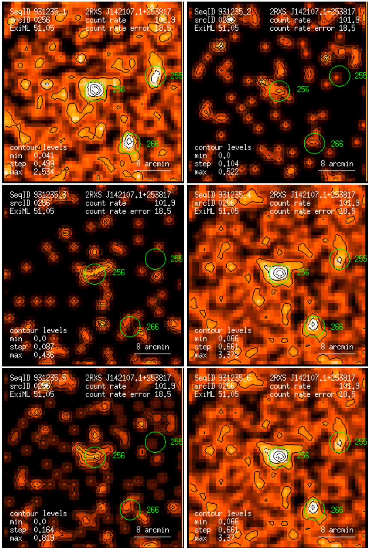
Figure 256: RASS 931235: detection 0256: band rate images, Gaussian filter: (1) PSPC channels 11 – 41, (2) 52 – 90, (3) 91 – 201, (4) 11 – 235, (5) 52 – 201, (6) 11 – 201. Broad band rates in counts/ks. Band rate contour levels in counts/ks/arcmin 2 .
