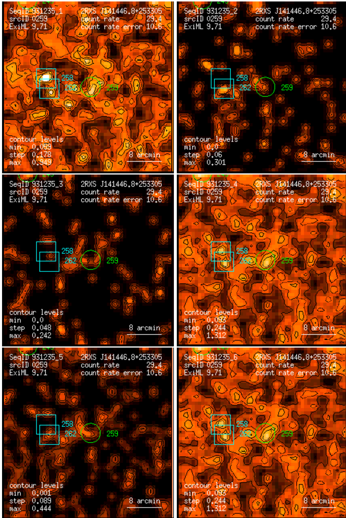
Figure 259: RASS 931235: detection 0259: band rate images, Gaussian filter: (1) PSPC channels 11 – 41, (2) 52 – 90, (3) 91 – 201, (4) 11 – 235, (5) 52 – 201, (6) 11 – 201. Broad band rates in counts/ks. Band rate contour levels in counts/ks/arcmin 2 .
