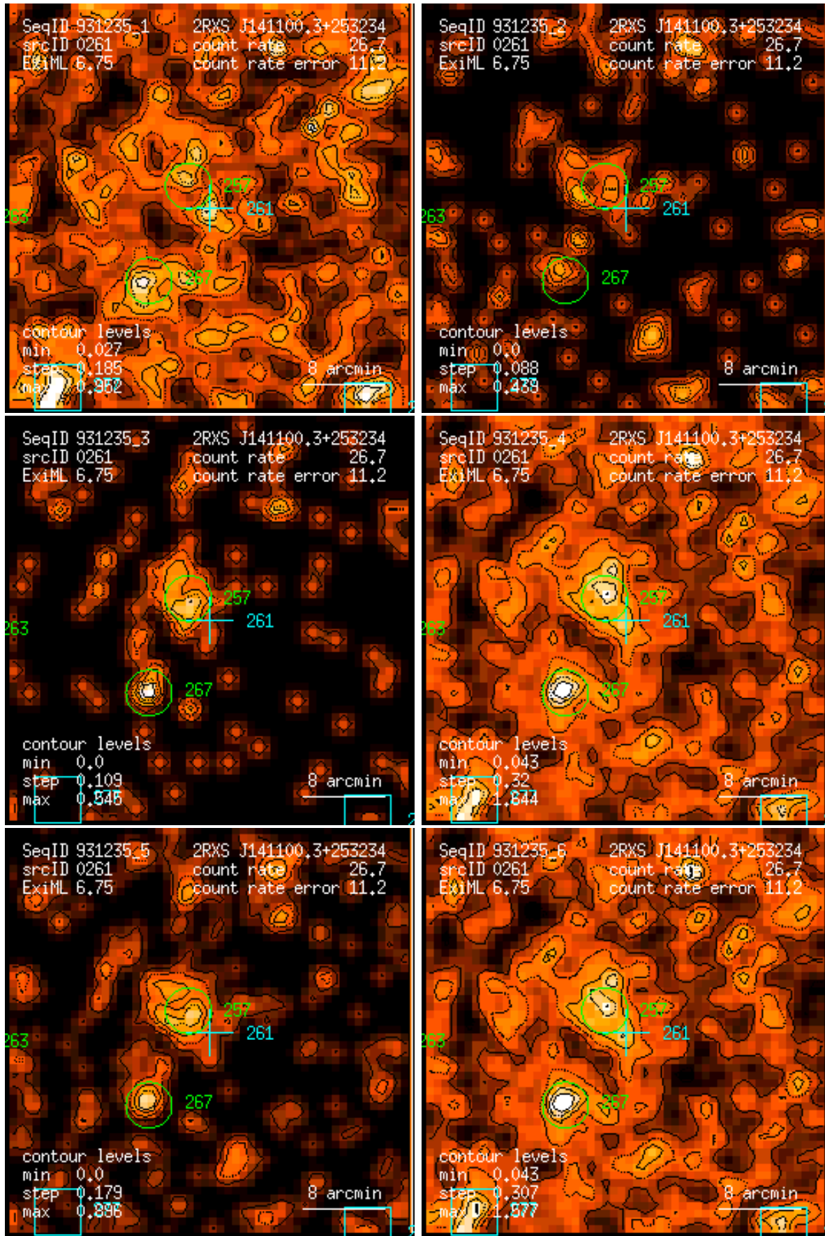
Figure 261: RASS 931235: detection 0261: band rate images, Gaussian filter: (1) PSPC channels 11 – 41, (2) 52 – 90, (3) 91 – 201, (4) 11 – 235, (5) 52 – 201, (6) 11 – 201. Broad band rates in counts/ks. Band rate contour levels in counts/ks/arcmin 2 .
