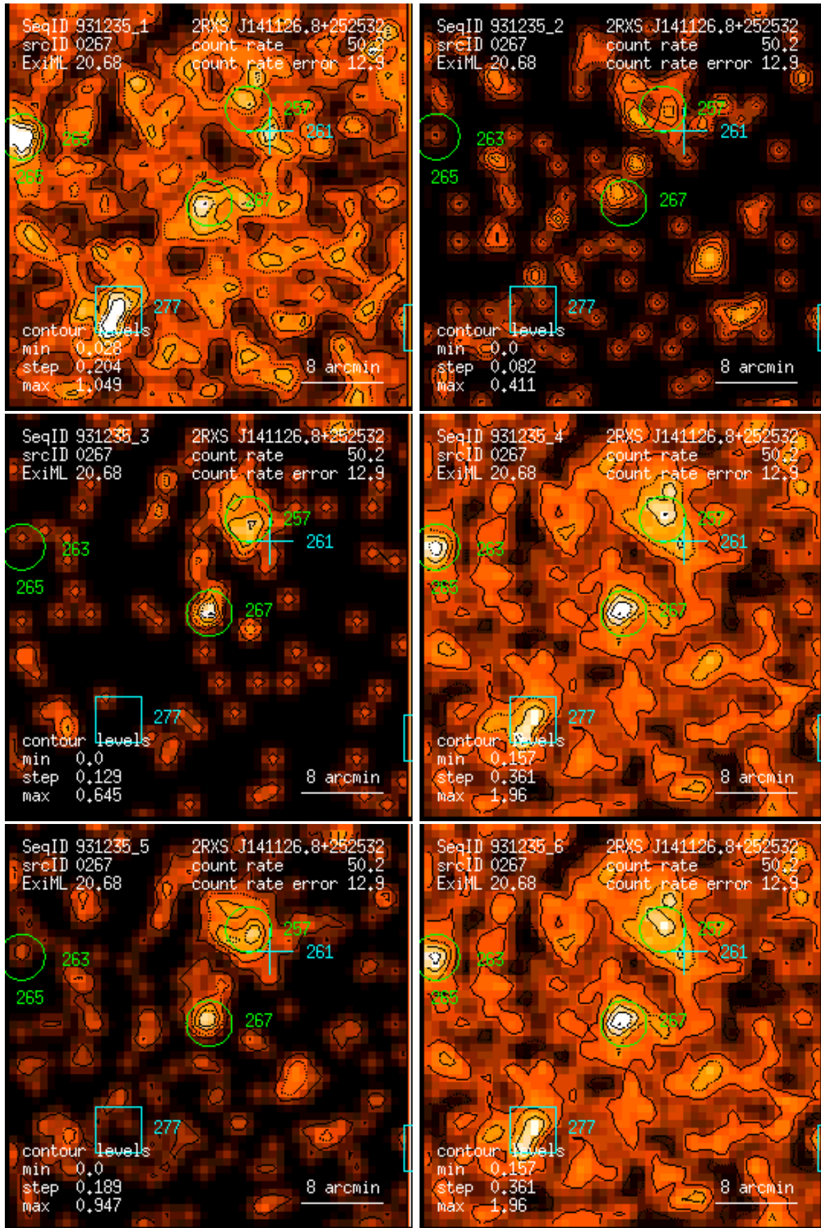
Figure 267: RASS 931235: detection 0267: band rate images, Gaussian filter: (1) PSPC channels 11 – 41, (2) 52 – 90, (3) 91 – 201, (4) 11 – 235, (5) 52 – 201, (6) 11 – 201. Broad band rates in counts/ks. Band rate contour levels in counts/ks/arcmin 2 .
