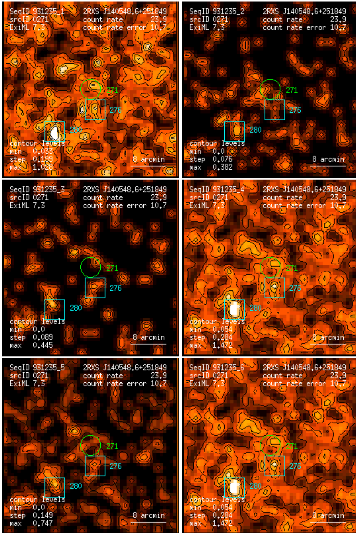
Figure 271: RASS 931235: detection 0271: band rate images, Gaussian filter: (1) PSPC channels 11 – 41, (2) 52 – 90, (3) 91 – 201, (4) 11 – 235, (5) 52 – 201, (6) 11 – 201. Broad band rates in counts/ks. Band rate contour levels in counts/ks/arcmin 2 .
