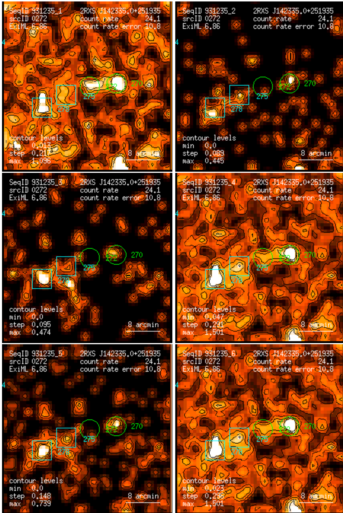
Figure 272: RASS 931235: detection 0272: band rate images, Gaussian filter: (1) PSPC channels 11 – 41, (2) 52 – 90, (3) 91 – 201, (4) 11 – 235, (5) 52 – 201, (6) 11 – 201. Broad band rates in counts/ks. Band rate contour levels in counts/ks/arcmin 2 .
