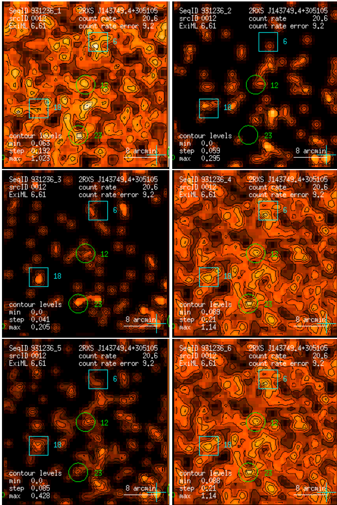
Figure 12: RASS 931236: detection 0012: band rate images, Gaussian filter: (1) PSPC channels 11 – 41, (2) 52 – 90, (3) 91 – 201, (4) 11 – 235, (5) 52 – 201, (6) 11 – 201. Broad band rates in counts/ks. Band rate contour levels in counts/ks/arcmin 2 .
