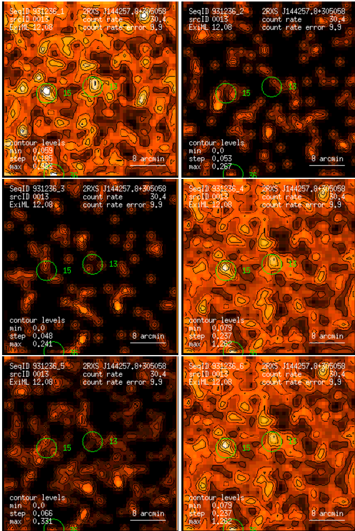
Figure 13: RASS 931236: detection 0013: band rate images, Gaussian filter: (1) PSPC channels 11 – 41, (2) 52 – 90, (3) 91 – 201, (4) 11 – 235, (5) 52 – 201, (6) 11 – 201. Broad band rates in counts/ks. Band rate contour levels in counts/ks/arcmin 2 .
