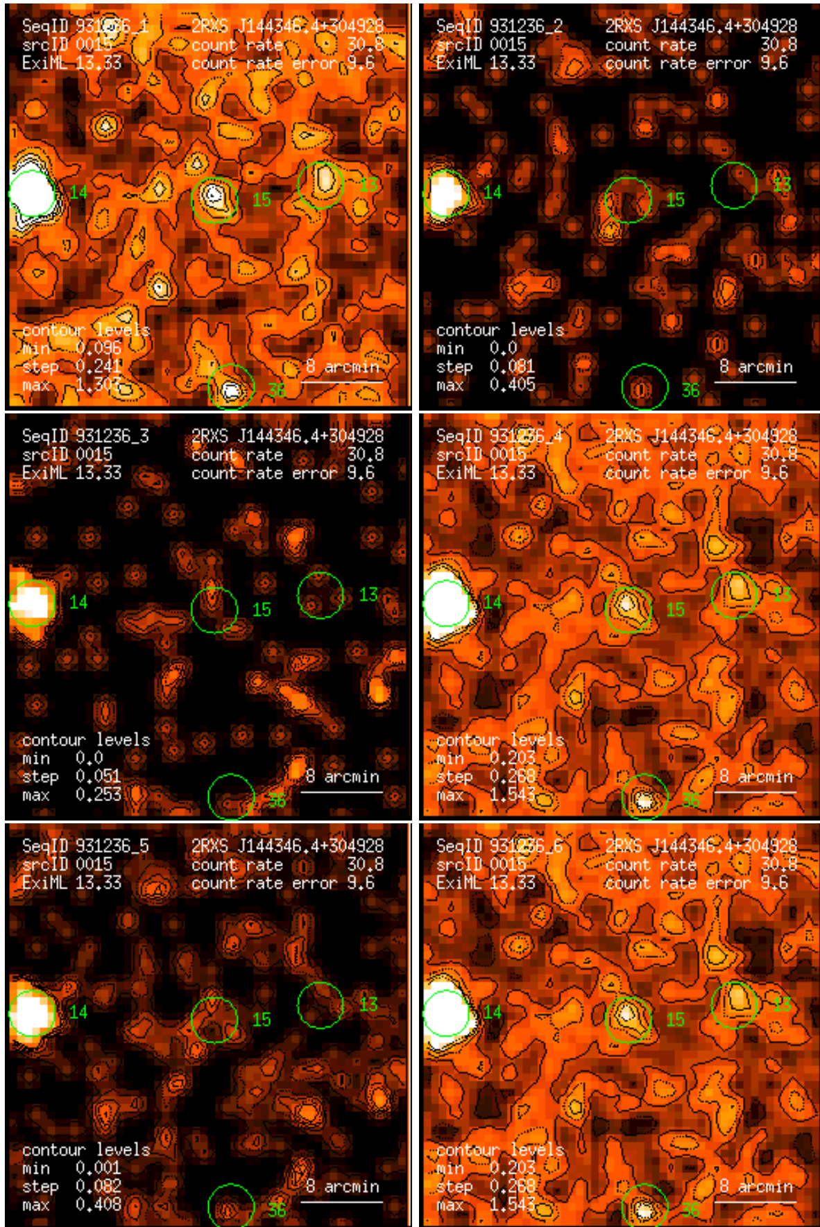
Figure 15: RASS 931236: detection 0015: band rate images, Gaussian filter: (1) PSPC channels 11 – 41, (2) 52 – 90, (3) 91 – 201, (4) 11 – 235, (5) 52 – 201, (6) 11 – 201. Broad band rates in counts/ks. Band rate contour levels in counts/ks/arcmin 2 .
