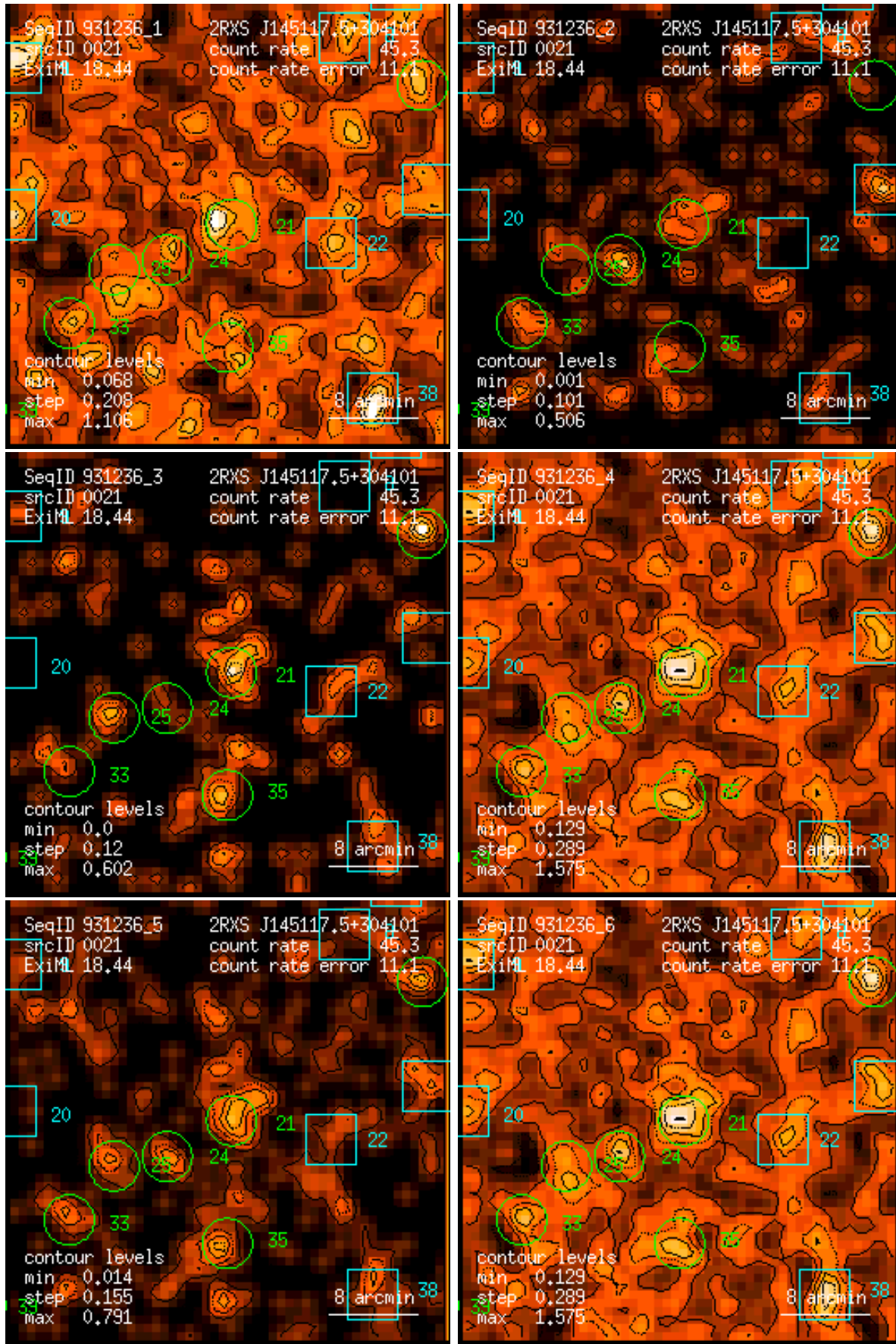
Figure 21: RASS 931236: detection 0021: band rate images, Gaussian filter: (1) PSPC channels 11 – 41, (2) 52 – 90, (3) 91 – 201, (4) 11 – 235, (5) 52 – 201, (6) 11 – 201. Broad band rates in counts/ks. Band rate contour levels in counts/ks/arcmin 2 .
