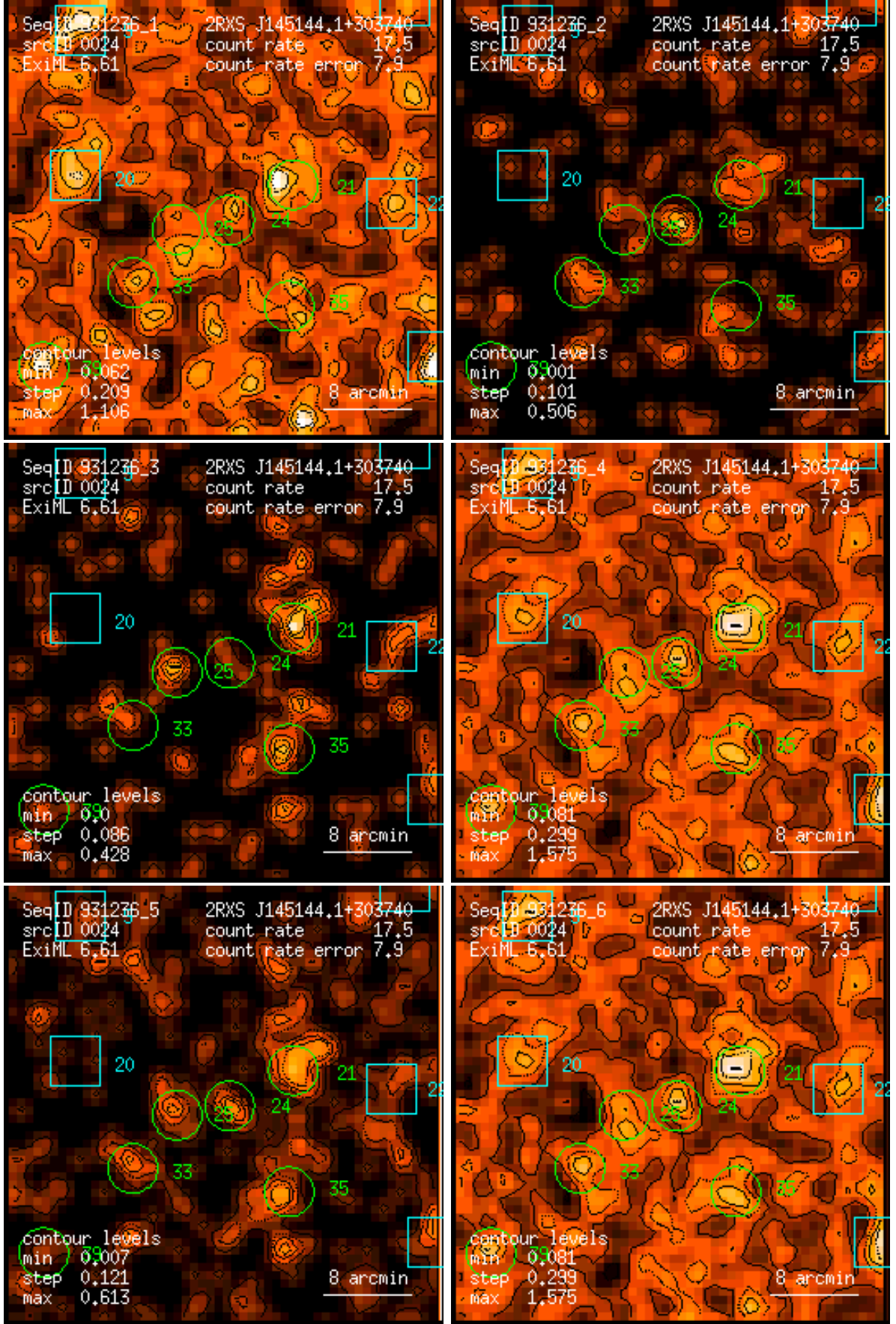
Figure 24: RASS 931236: detection 0024: band rate images, Gaussian filter: (1) PSPC channels 11 – 41, (2) 52 – 90, (3) 91 – 201, (4) 11 – 235, (5) 52 – 201, (6) 11 – 201. Broad band rates in counts/ks. Band rate contour levels in counts/ks/arcmin 2 .
