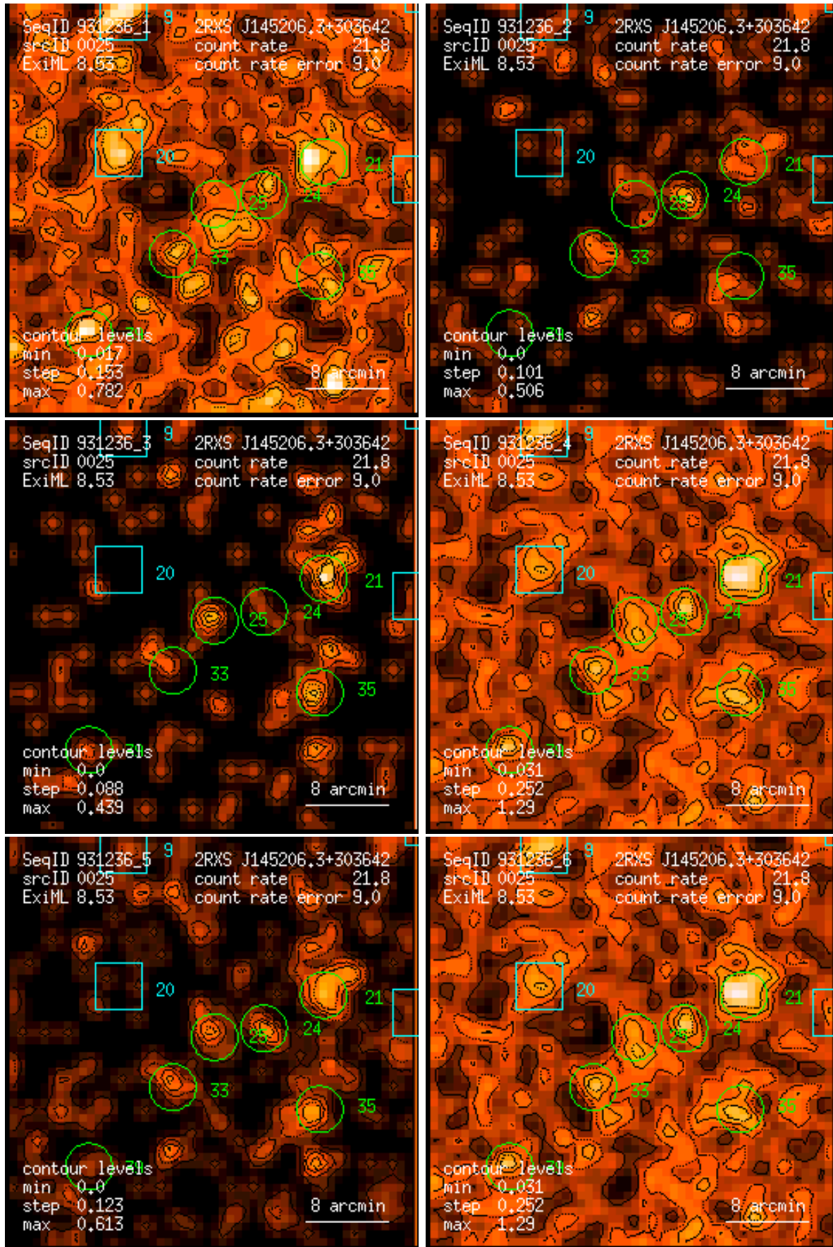
Figure 25: RASS 931236: detection 0025: band rate images, Gaussian filter: (1) PSPC channels 11 – 41, (2) 52 – 90, (3) 91 – 201, (4) 11 – 235, (5) 52 – 201, (6) 11 – 201. Broad band rates in counts/ks. Band rate contour levels in counts/ks/arcmin 2 .
