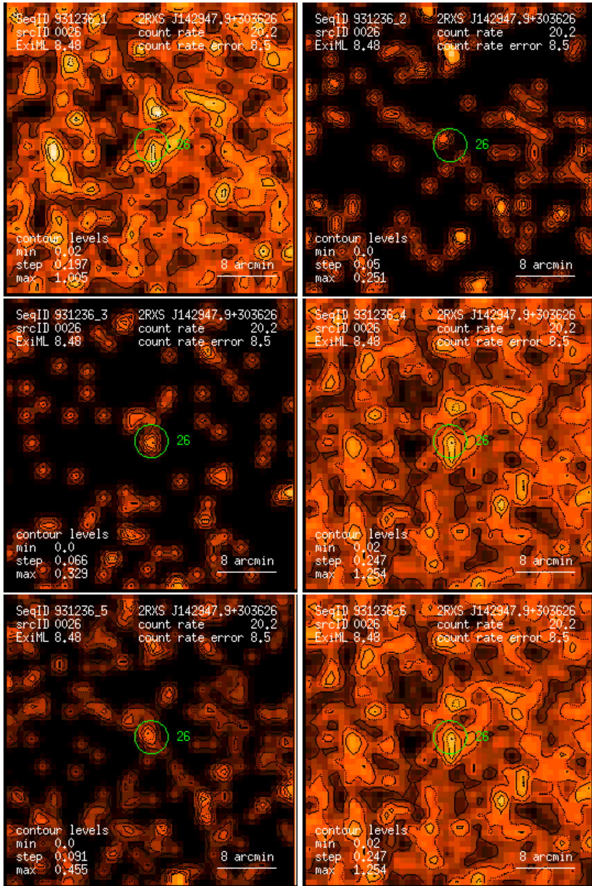
Figure 26: RASS 931236: detection 0026: band rate images, Gaussian filter: (1) PSPC channels 11 – 41, (2) 52 – 90, (3) 91 – 201, (4) 11 – 235, (5) 52 – 201, (6) 11 – 201. Broad band rates in counts/ks. Band rate contour levels in counts/ks/arcmin 2 .
