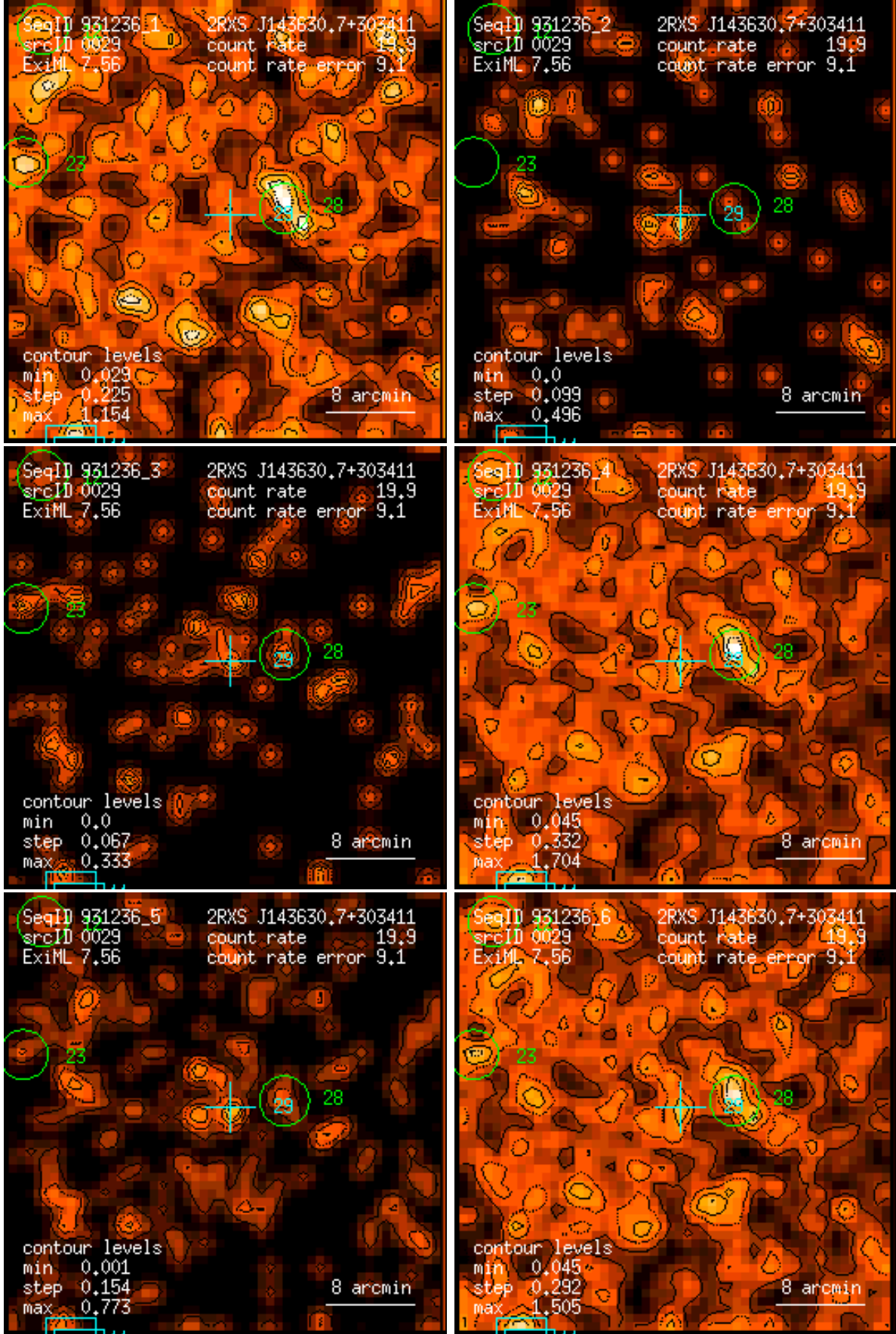
Figure 29: RASS 931236: detection 0029: band rate images, Gaussian filter: (1) PSPC channels 11 – 41, (2) 52 – 90, (3) 91 – 201, (4) 11 – 235, (5) 52 – 201, (6) 11 – 201. Broad band rates in counts/ks. Band rate contour levels in counts/ks/arcmin 2 .
