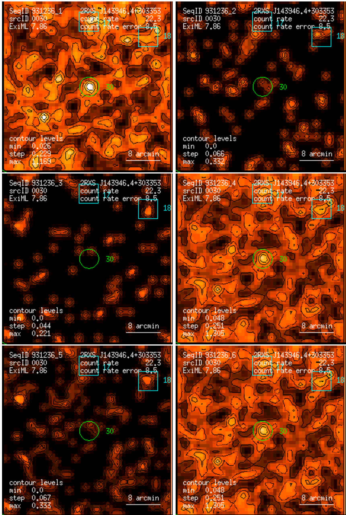
Figure 30: RASS 931236: detection 0030: band rate images, Gaussian filter: (1) PSPC channels 11 – 41, (2) 52 – 90, (3) 91 – 201, (4) 11 – 235, (5) 52 – 201, (6) 11 – 201. Broad band rates in counts/ks. Band rate contour levels in counts/ks/arcmin 2 .
