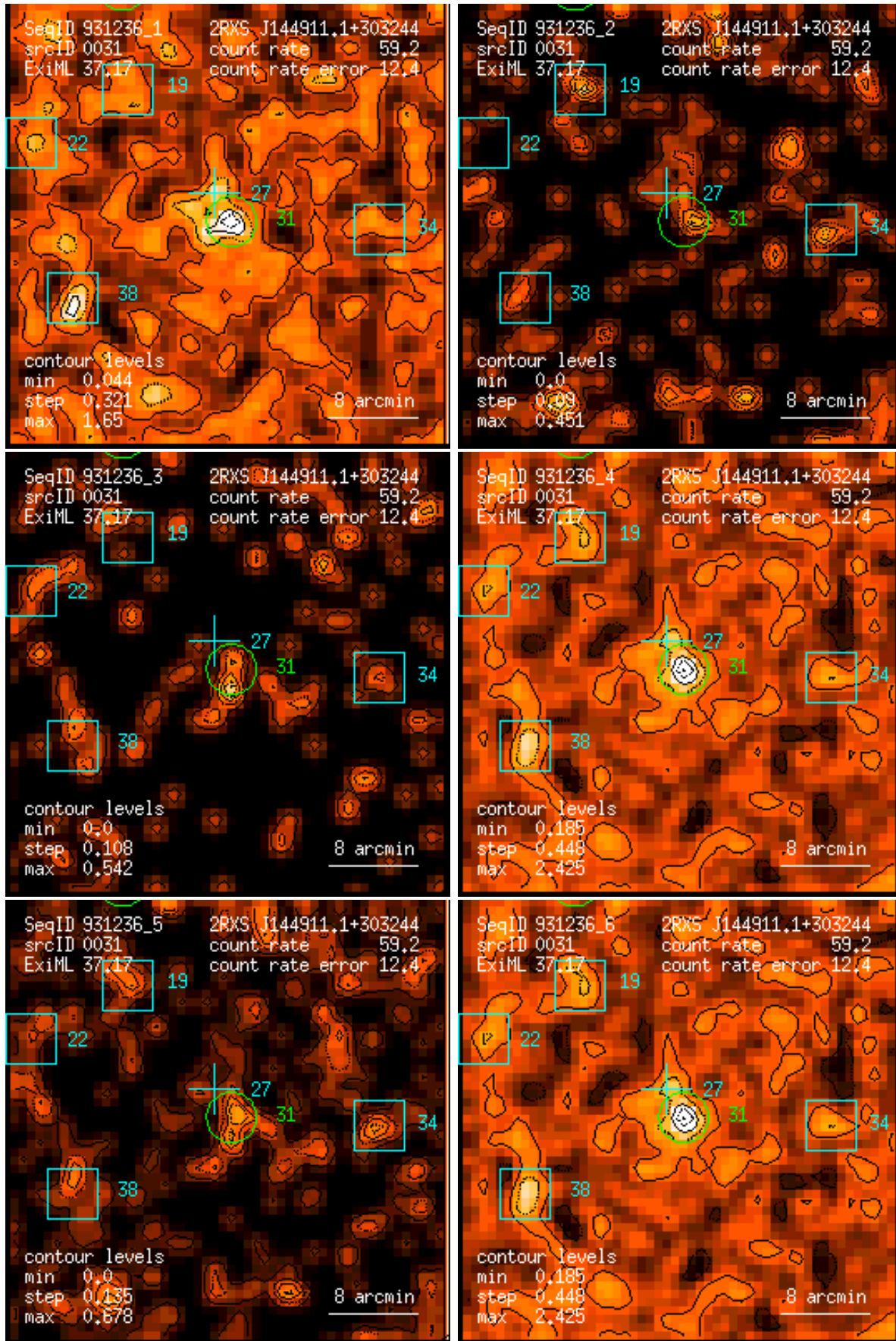
Figure 31: RASS 931236: detection 0031: band rate images, Gaussian filter: (1) PSPC channels 11 – 41, (2) 52 – 90, (3) 91 – 201, (4) 11 – 235, (5) 52 – 201, (6) 11 – 201. Broad band rates in counts/ks. Band rate contour levels in counts/ks/arcmin 2 .
