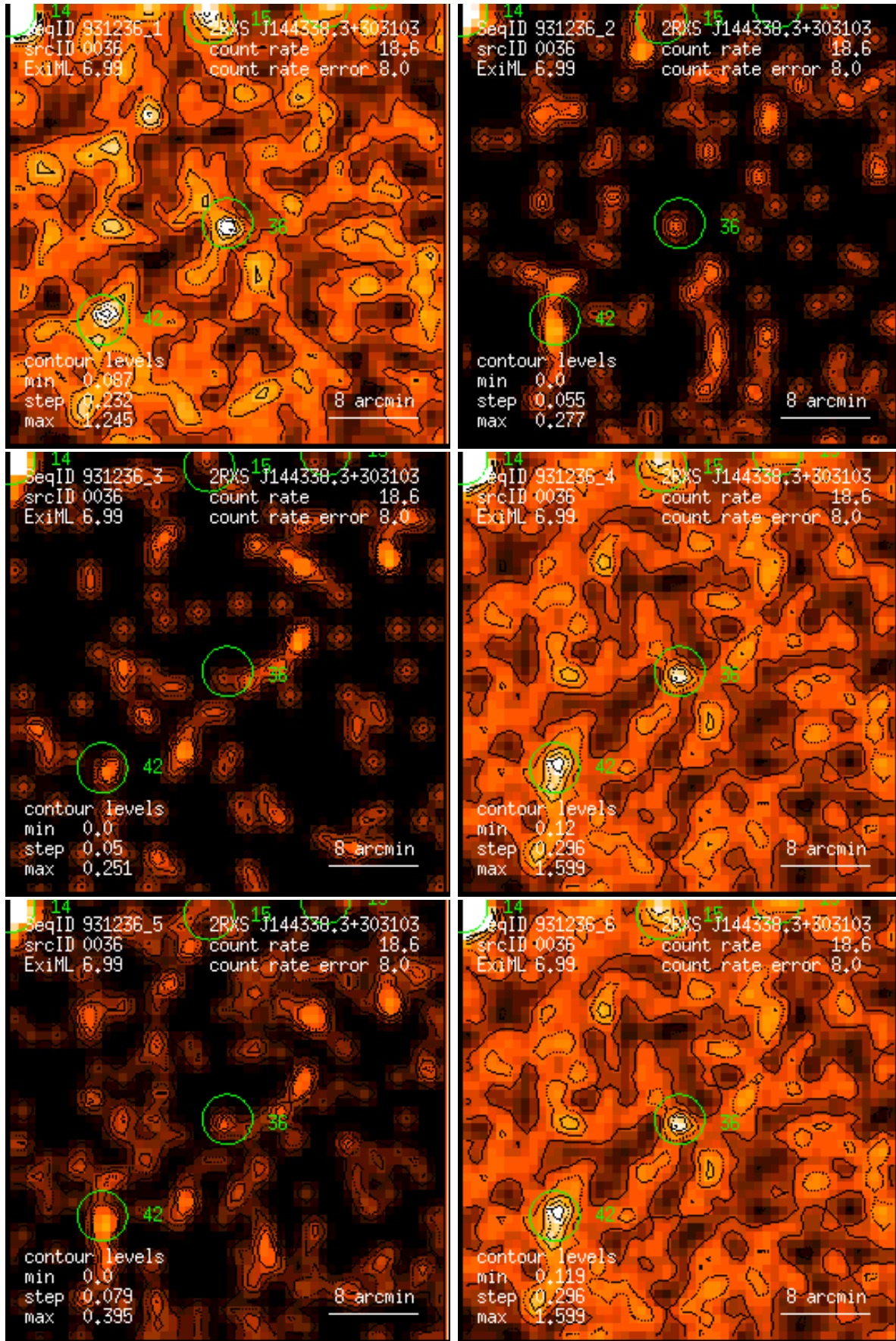
Figure 36: RASS 931236: detection 0036: band rate images, Gaussian filter: (1) PSPC channels 11 – 41, (2) 52 – 90, (3) 91 – 201, (4) 11 – 235, (5) 52 – 201, (6) 11 – 201. Broad band rates in counts/ks. Band rate contour levels in counts/ks/arcmin 2 .
