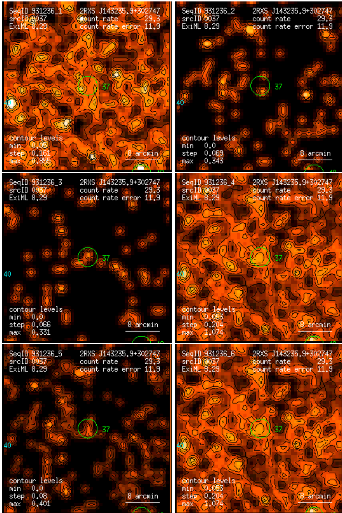
Figure 37: RASS 931236: detection 0037: band rate images, Gaussian filter: (1) PSPC channels 11 – 41, (2) 52 – 90, (3) 91 – 201, (4) 11 – 235, (5) 52 – 201, (6) 11 – 201. Broad band rates in counts/ks. Band rate contour levels in counts/ks/arcmin 2 .
