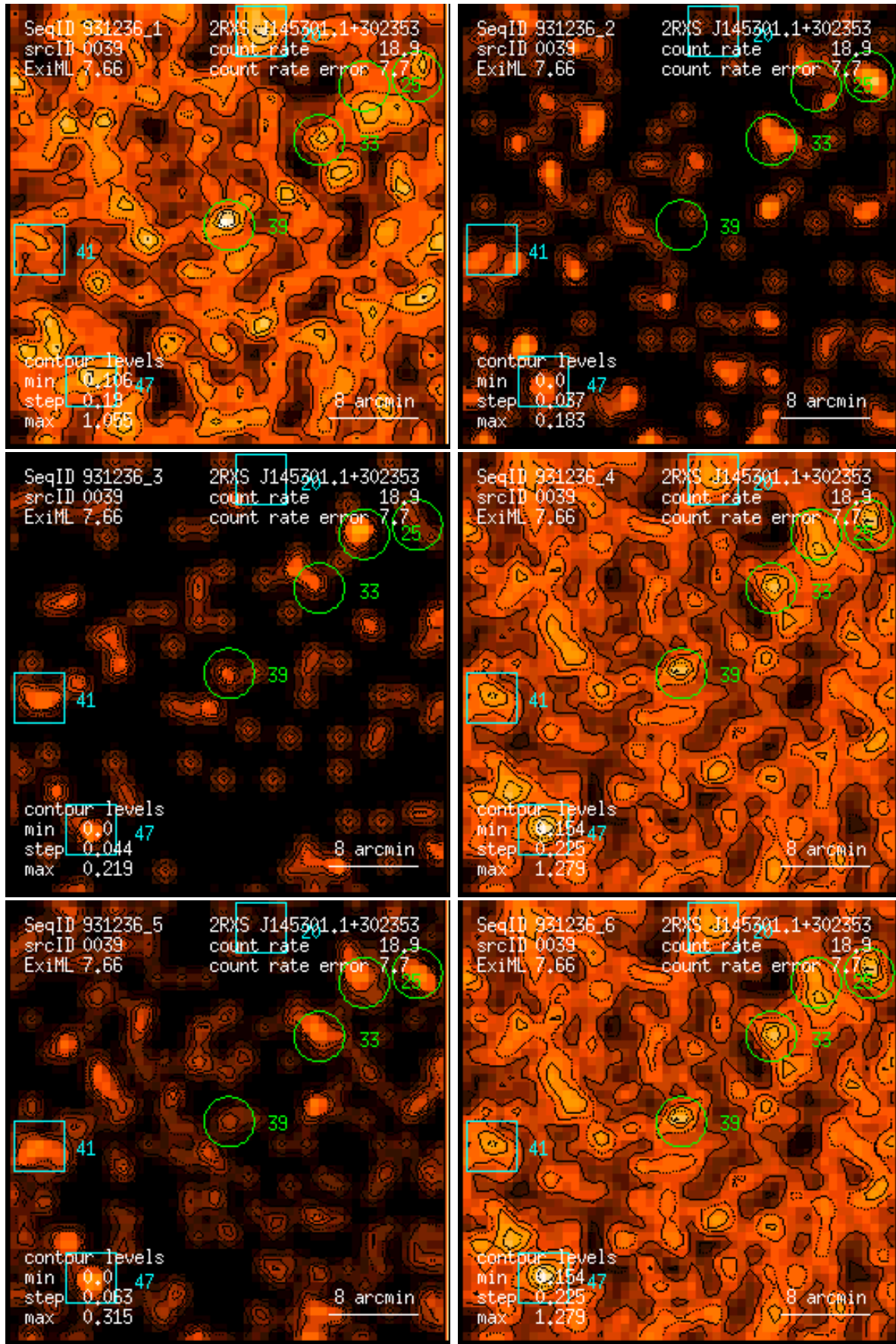
Figure 39: RASS 931236: detection 0039: band rate images, Gaussian filter: (1) PSPC channels 11 – 41, (2) 52 – 90, (3) 91 – 201, (4) 11 – 235, (5) 52 – 201, (6) 11 – 201. Broad band rates in counts/ks. Band rate contour levels in counts/ks/arcmin 2 .
