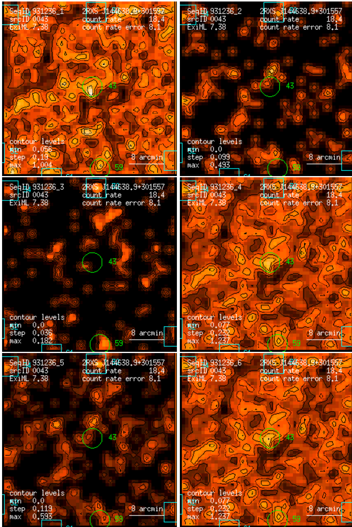
Figure 43: RASS 931236: detection 0043: band rate images, Gaussian filter: (1) PSPC channels 11 – 41, (2) 52 – 90, (3) 91 – 201, (4) 11 – 235, (5) 52 – 201, (6) 11 – 201. Broad band rates in counts/ks. Band rate contour levels in counts/ks/arcmin 2 .
