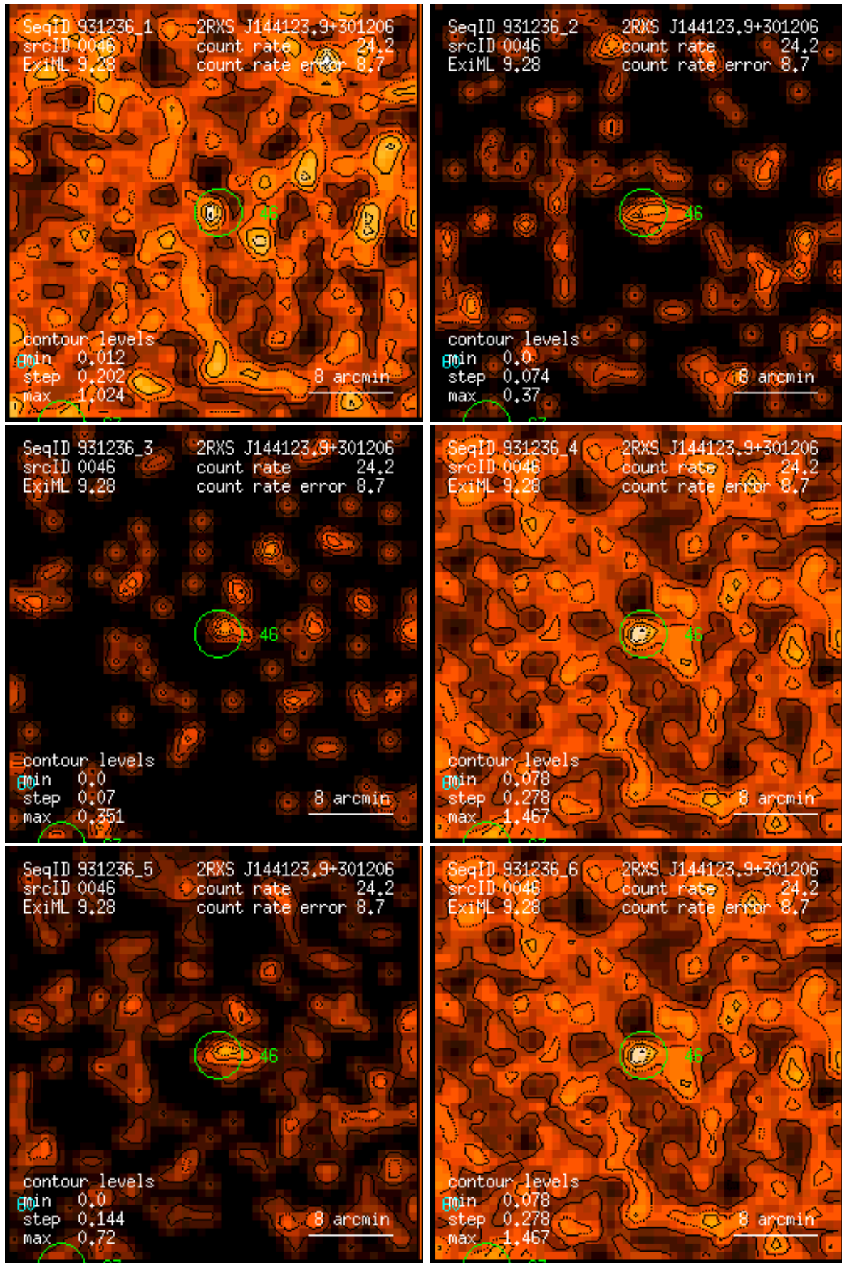
Figure 46: RASS 931236: detection 0046: band rate images, Gaussian filter: (1) PSPC channels 11 – 41, (2) 52 – 90, (3) 91 – 201, (4) 11 – 235, (5) 52 – 201, (6) 11 – 201. Broad band rates in counts/ks. Band rate contour levels in counts/ks/arcmin 2 .
