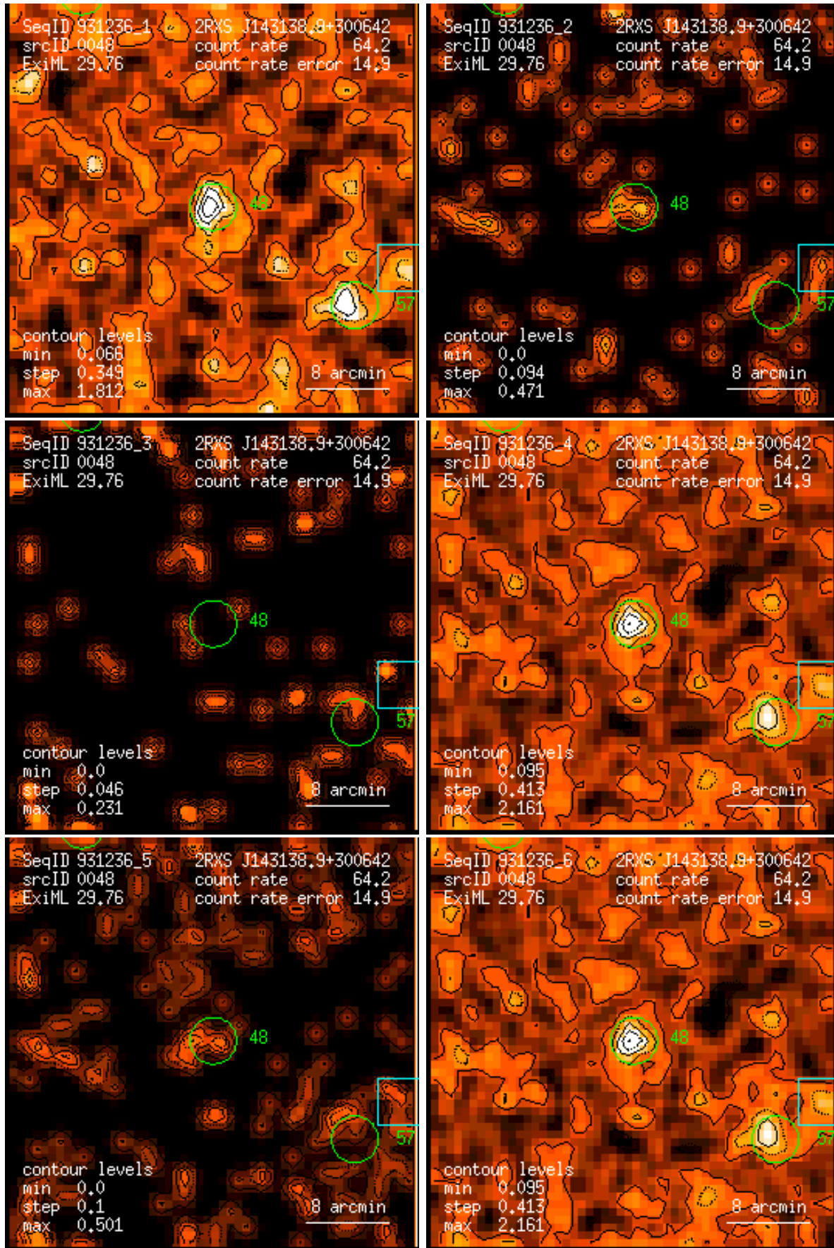
Figure 48: RASS 931236: detection 0048: band rate images, Gaussian filter: (1) PSPC channels 11 – 41, (2) 52 – 90, (3) 91 – 201, (4) 11 – 235, (5) 52 – 201, (6) 11 – 201. Broad band rates in counts/ks. Band rate contour levels in counts/ks/arcmin 2 .
