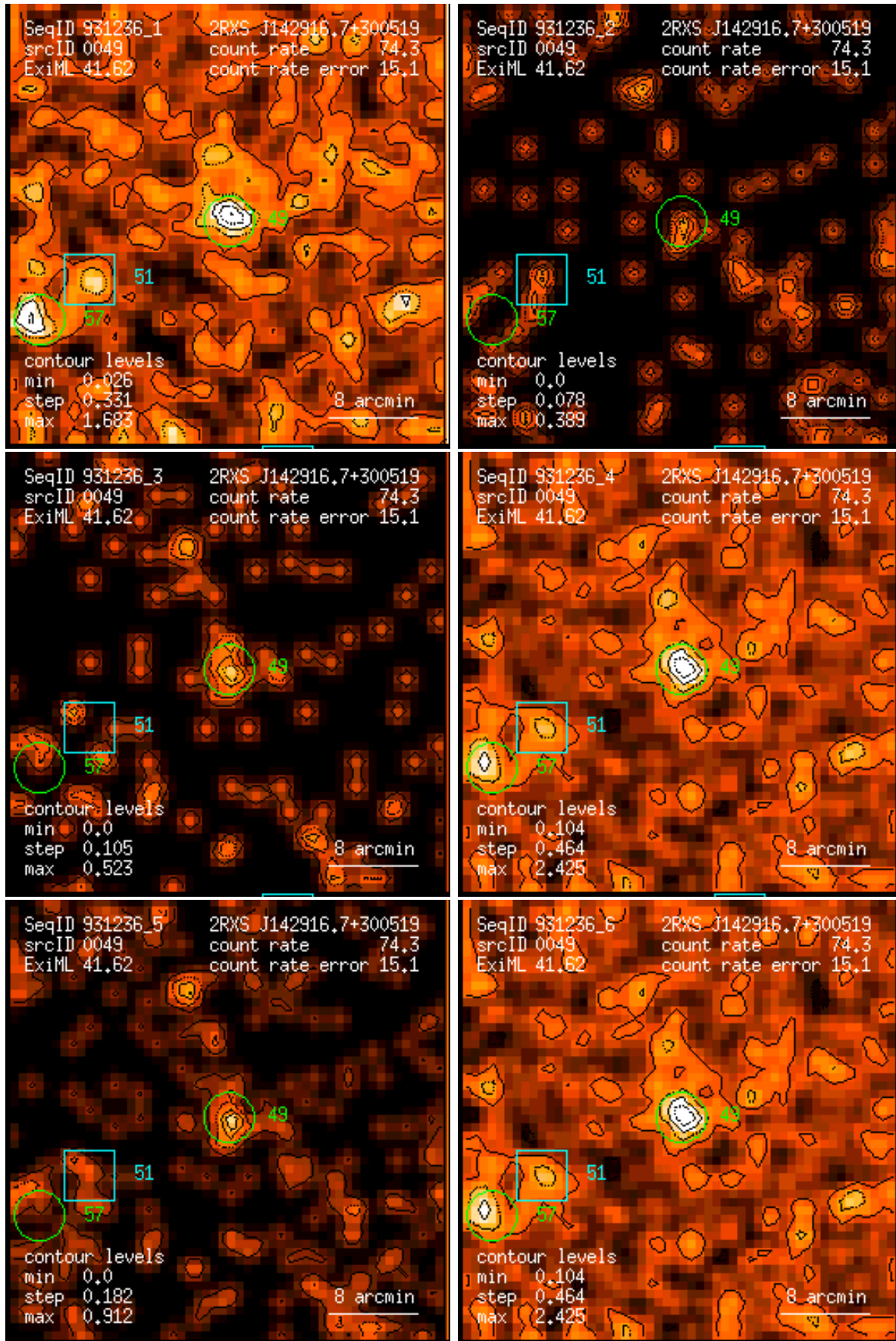
Figure 49: RASS 931236: detection 0049: band rate images, Gaussian filter: (1) PSPC channels 11 – 41, (2) 52 – 90, (3) 91 – 201, (4) 11 – 235, (5) 52 – 201, (6) 11 – 201. Broad band rates in counts/ks. Band rate contour levels in counts/ks/arcmin 2 .
