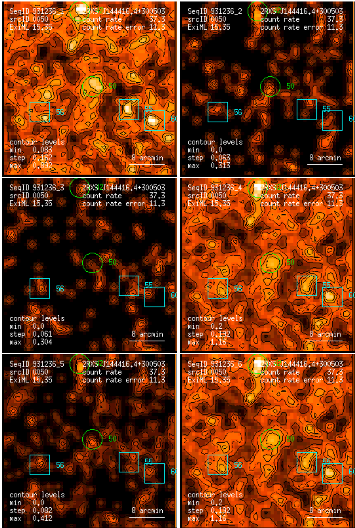
Figure 50: RASS 931236: detection 0050: band rate images, Gaussian filter: (1) PSPC channels 11 – 41, (2) 52 – 90, (3) 91 – 201, (4) 11 – 235, (5) 52 – 201, (6) 11 – 201. Broad band rates in counts/ks. Band rate contour levels in counts/ks/arcmin 2 .
