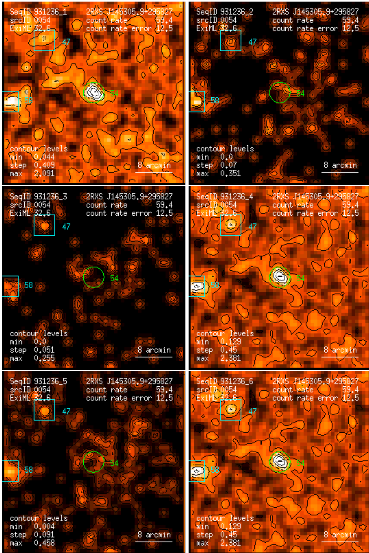
Figure 54: RASS 931236: detection 0054: band rate images, Gaussian filter: (1) PSPC channels 11 – 41, (2) 52 – 90, (3) 91 – 201, (4) 11 – 235, (5) 52 – 201, (6) 11 – 201. Broad band rates in counts/ks. Band rate contour levels in counts/ks/arcmin 2 .
