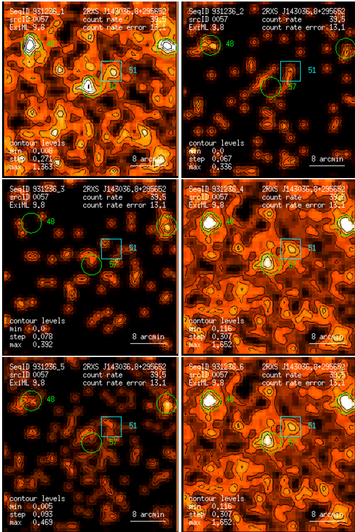
Figure 57: RASS 931236: detection 0057: band rate images, Gaussian filter: (1) PSPC channels 11 – 41, (2) 52 – 90, (3) 91 – 201, (4) 11 – 235, (5) 52 – 201, (6) 11 – 201. Broad band rates in counts/ks. Band rate contour levels in counts/ks/arcmin 2 .
