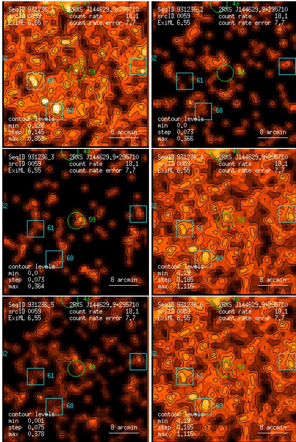
Figure 59: RASS 931236: detection 0059: band rate images, Gaussian filter: (1) PSPC channels 11 – 41, (2) 52 – 90, (3) 91 – 201, (4) 11 – 235, (5) 52 – 201, (6) 11 – 201. Broad band rates in counts/ks. Band rate contour levels in counts/ks/arcmin 2 .
