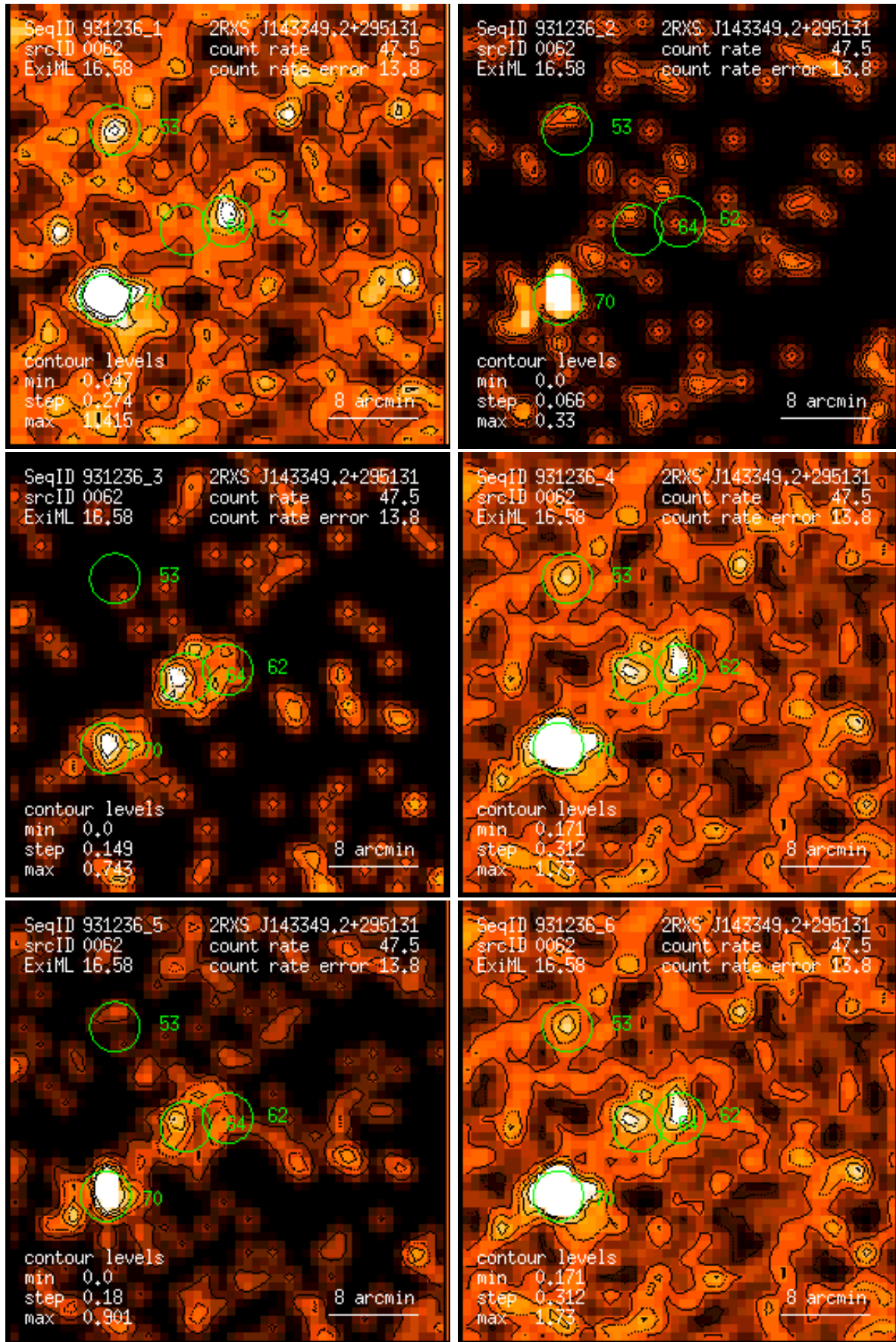
Figure 62: RASS 931236: detection 0062: band rate images, Gaussian filter: (1) PSPC channels 11 – 41, (2) 52 – 90, (3) 91 – 201, (4) 11 – 235, (5) 52 – 201, (6) 11 – 201. Broad band rates in counts/ks. Band rate contour levels in counts/ks/arcmin 2 .
