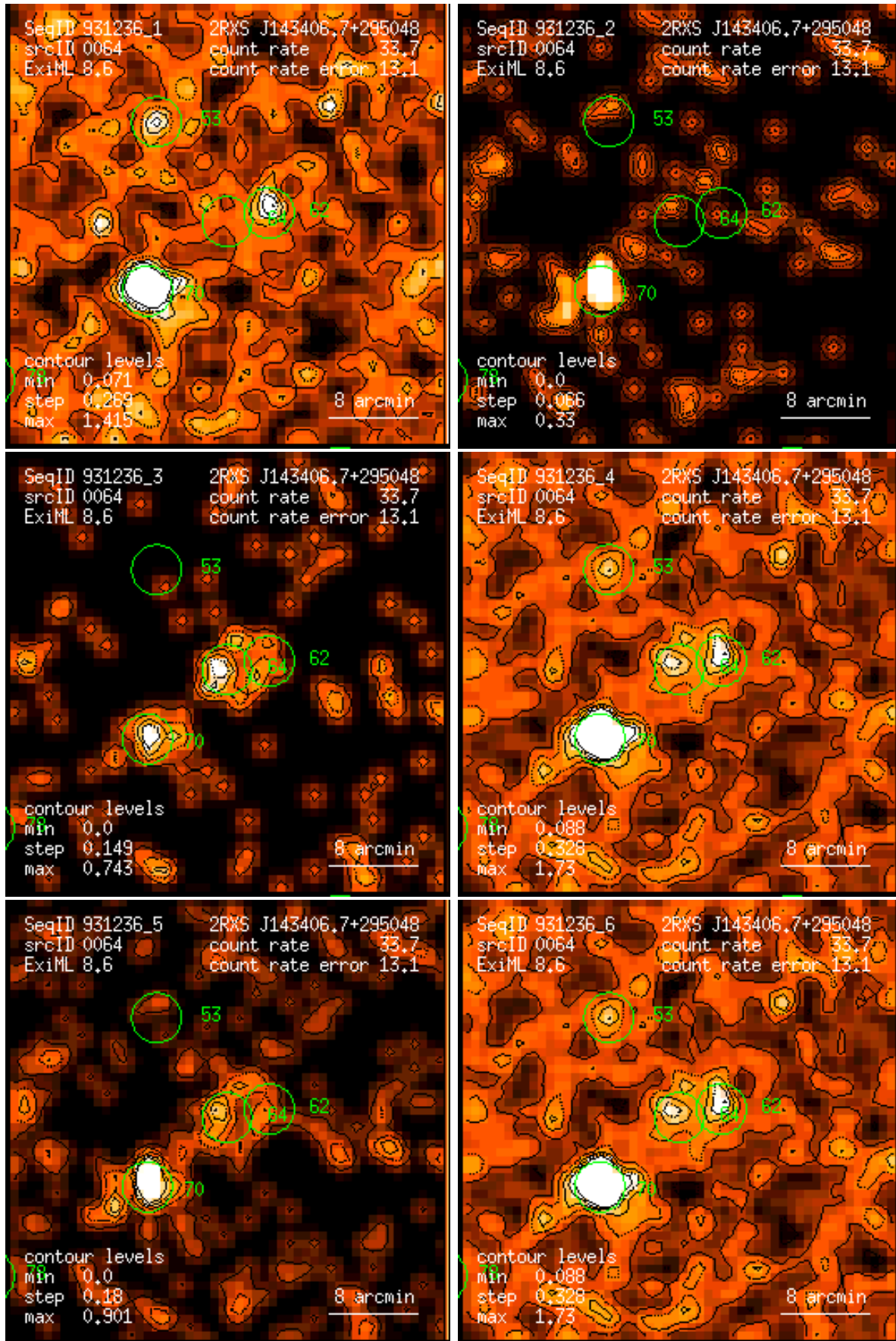
Figure 64: RASS 931236: detection 0064: band rate images, Gaussian filter: (1) PSPC channels 11 – 41, (2) 52 – 90, (3) 91 – 201, (4) 11 – 235, (5) 52 – 201, (6) 11 – 201. Broad band rates in counts/ks. Band rate contour levels in counts/ks/arcmin 2 .
