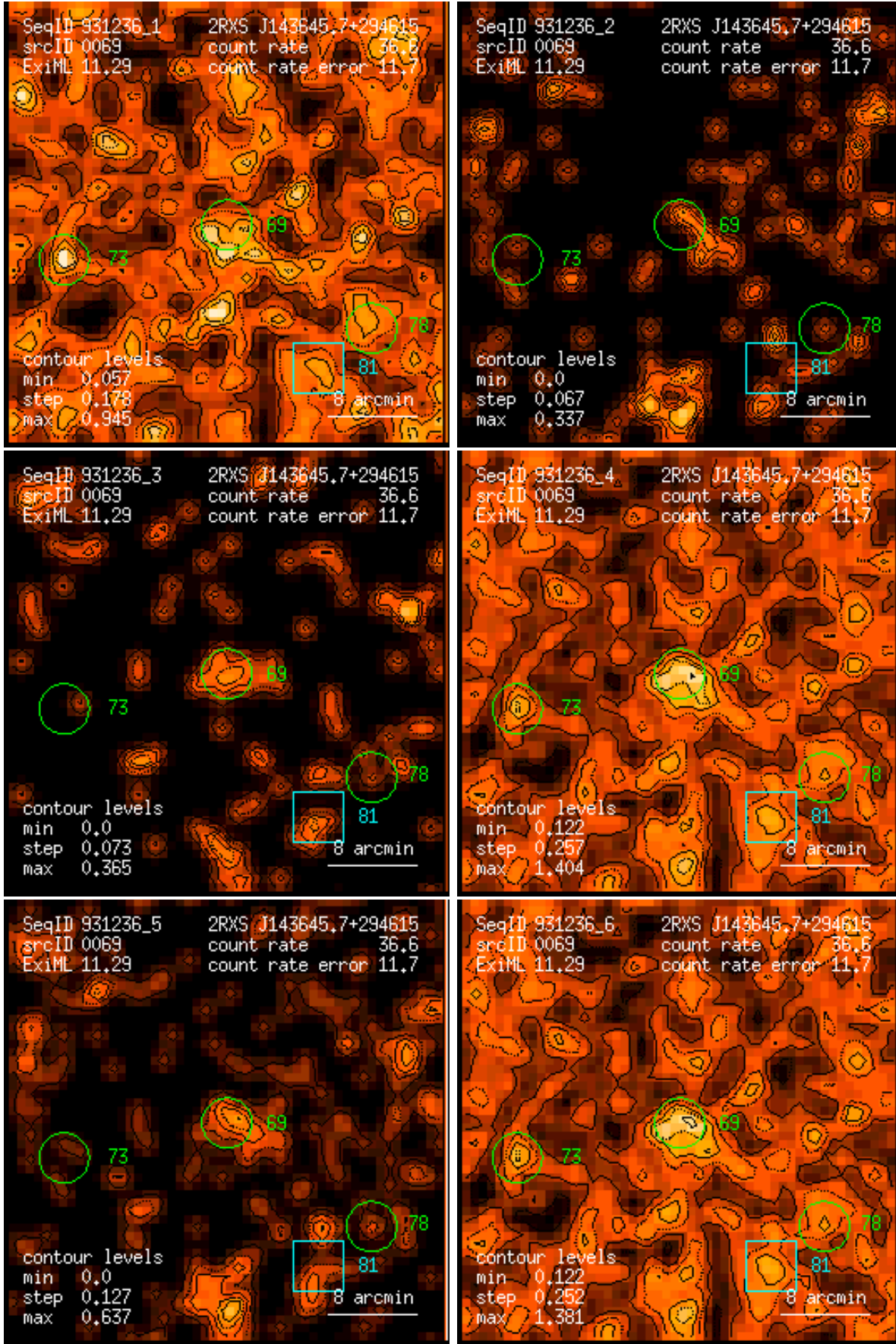
Figure 69: RASS 931236: detection 0069: band rate images, Gaussian filter: (1) PSPC channels 11 – 41, (2) 52 – 90, (3) 91 – 201, (4) 11 – 235, (5) 52 – 201, (6) 11 – 201. Broad band rates in counts/ks. Band rate contour levels in counts/ks/arcmin 2 .
