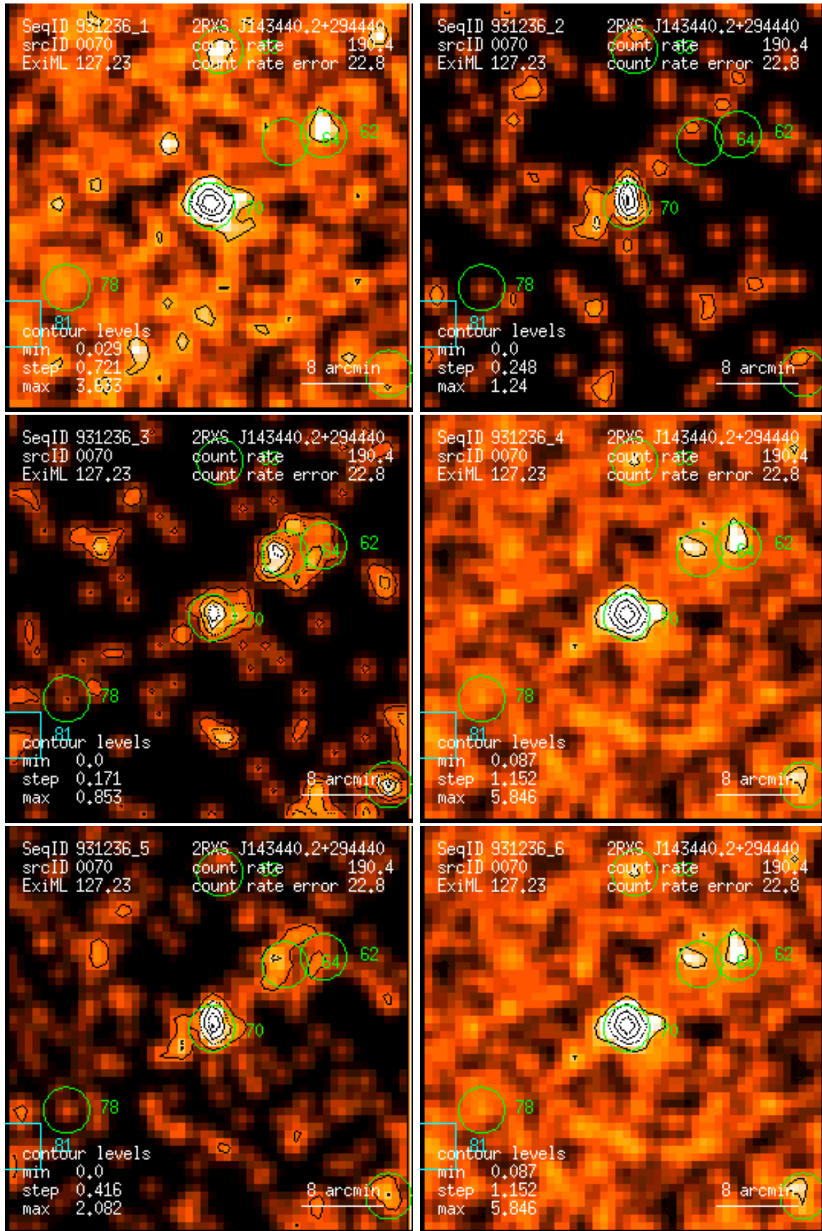
Figure 70: RASS 931236: detection 0070: band rate images, Gaussian filter: (1) PSPC channels 11 – 41, (2) 52 – 90, (3) 91 – 201, (4) 11 – 235, (5) 52 – 201, (6) 11 – 201. Broad band rates in counts/ks. Band rate contour levels in counts/ks/arcmin 2 .
